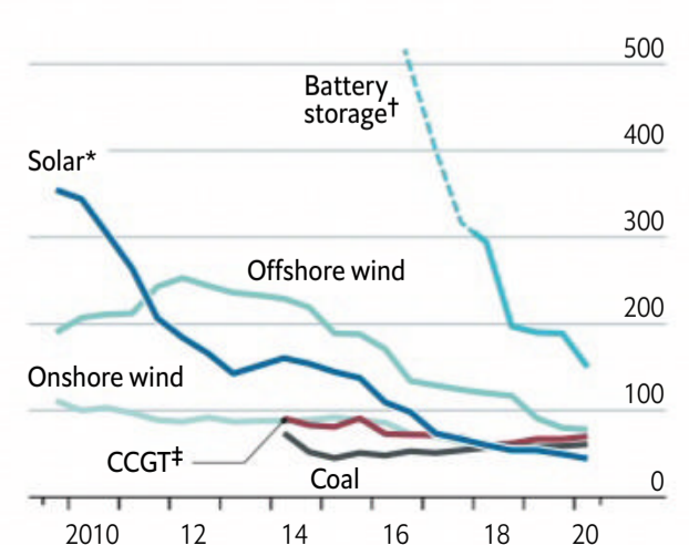
Levelised cost of energy, $ per MWh 2019 prices
