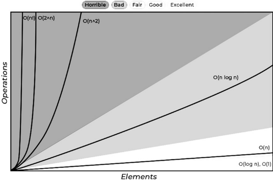
Figure 9-2. Big O Notation complexity over time chart
