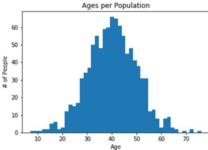
Figure 10-6. Histogram of centrally distributed age data
