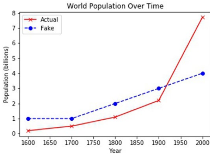
Figure 10-2. Multiline plot of population data
