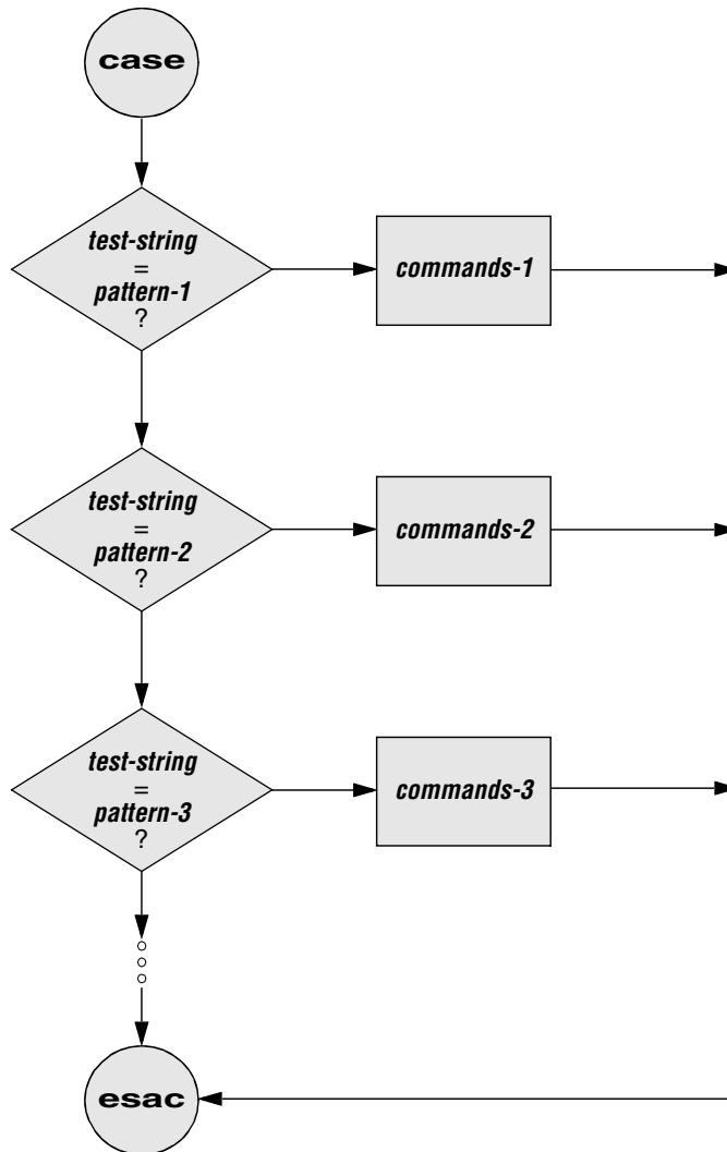
Figure 10-7 A case flowchart
