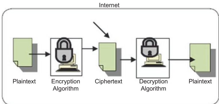
Fig. 11.1 Symmetric encryption
