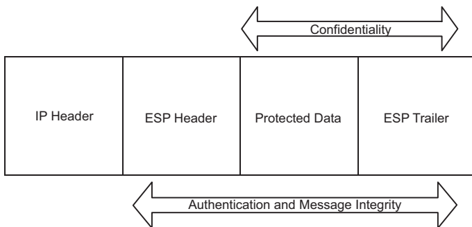
Fig. 17.9 IPsec's ESP protocol protection
