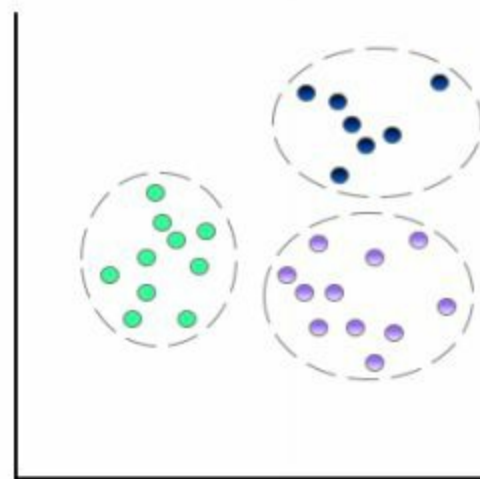
Clustered Data
