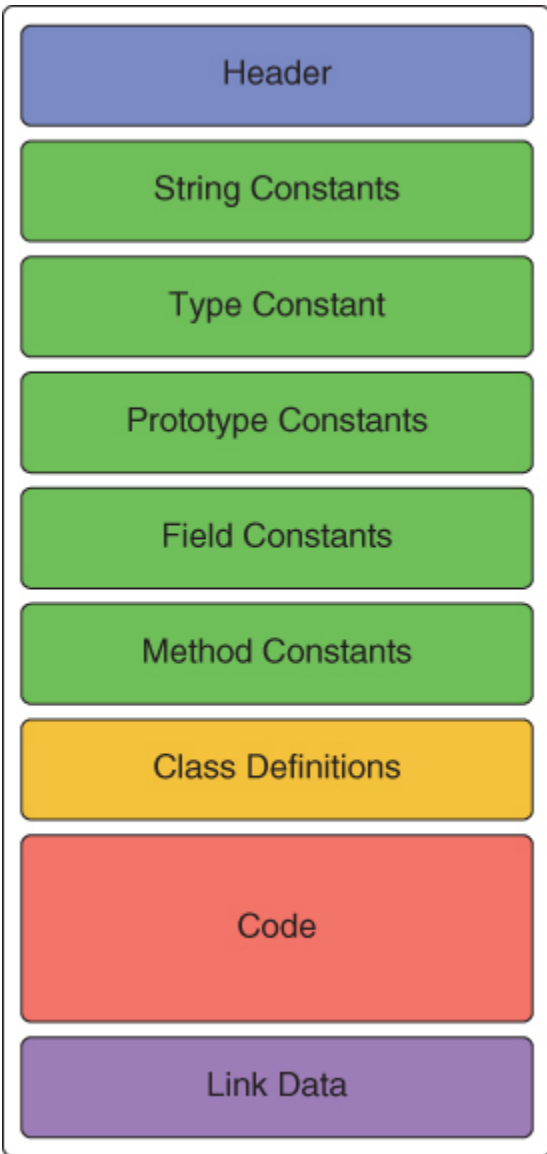
Figure 7.1 DEX File Structure
