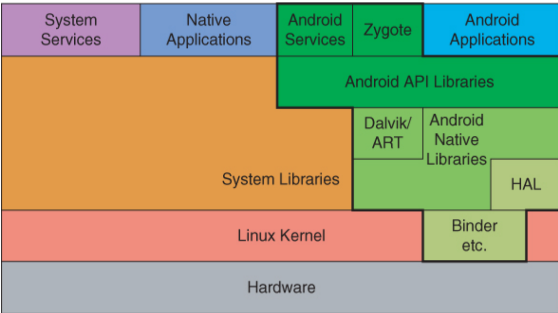
Figure 3.1 Android Layer Cake
