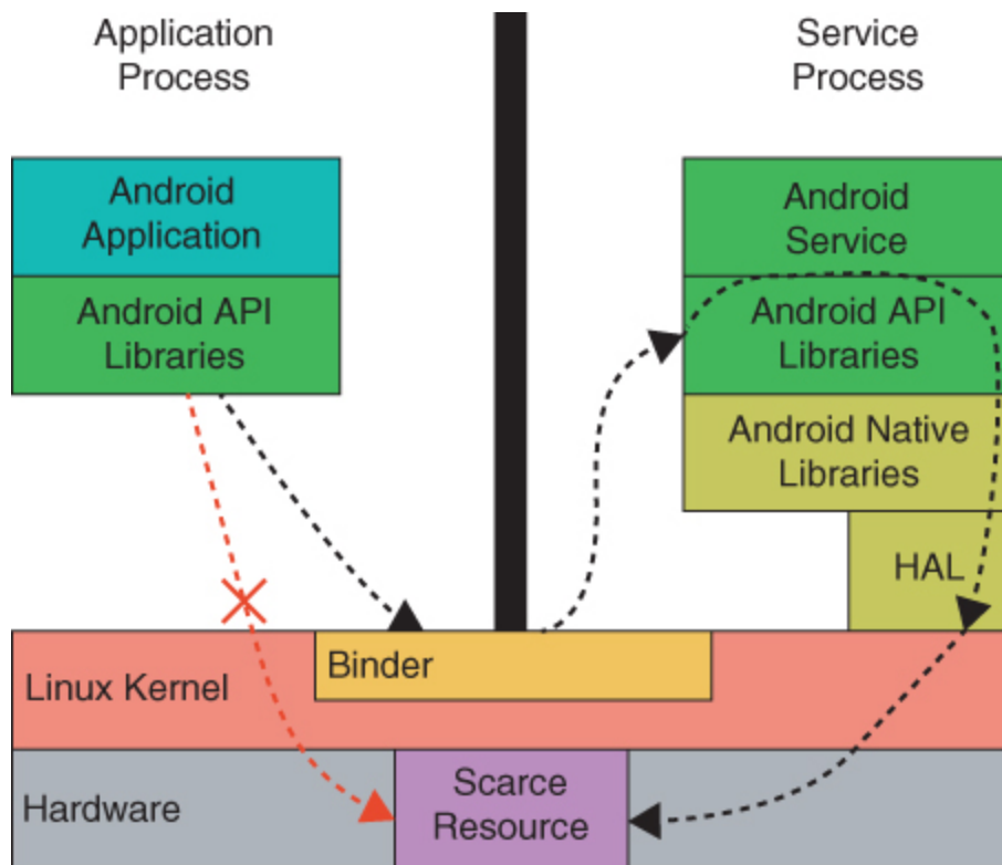
Figure 3.2 The Android System Model
