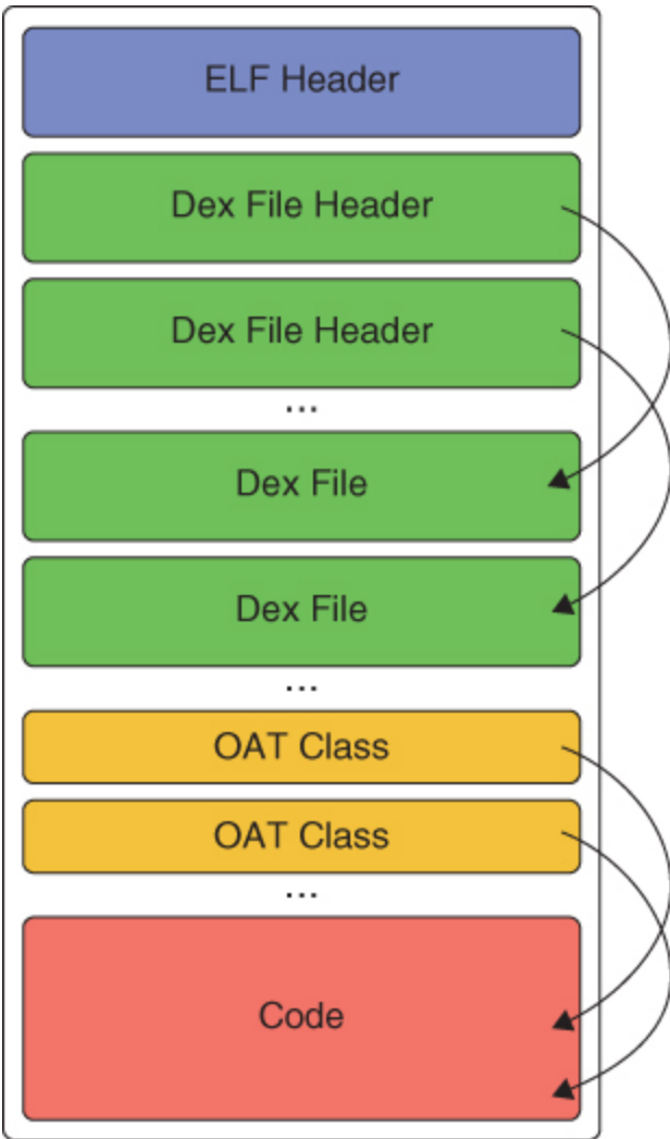
Figure 7.2 OAT File Structure
