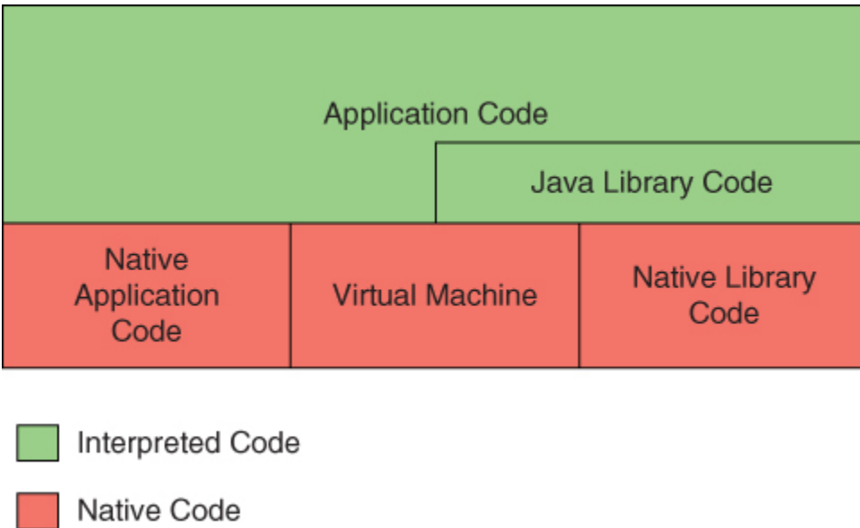
Figure 9.2 Interpreted and Native Code
