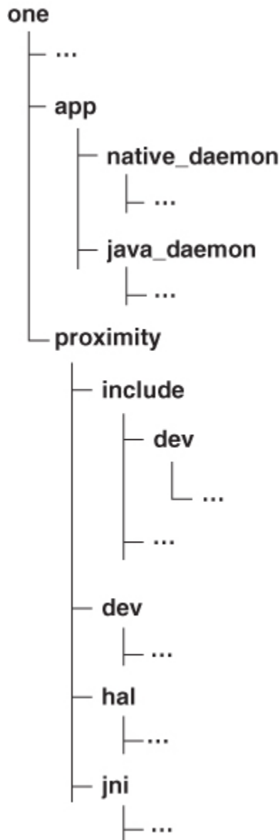
Figure 8.2 HAL Directory Structure
