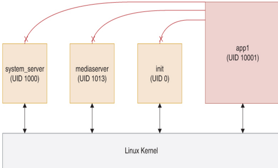
Figure 5.2 Android Process Sandbox
