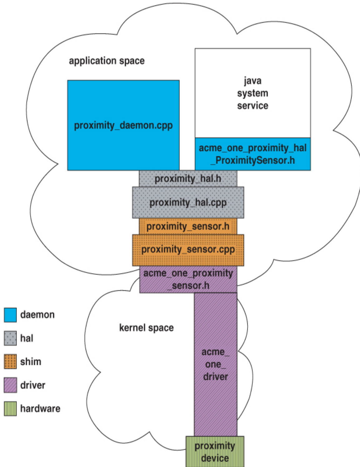
Figure 8.1 HAL Layer Structure
