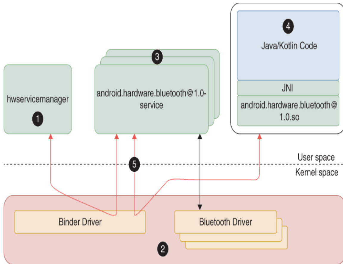
Figure 10.1 HIDL High-Level Architecture
