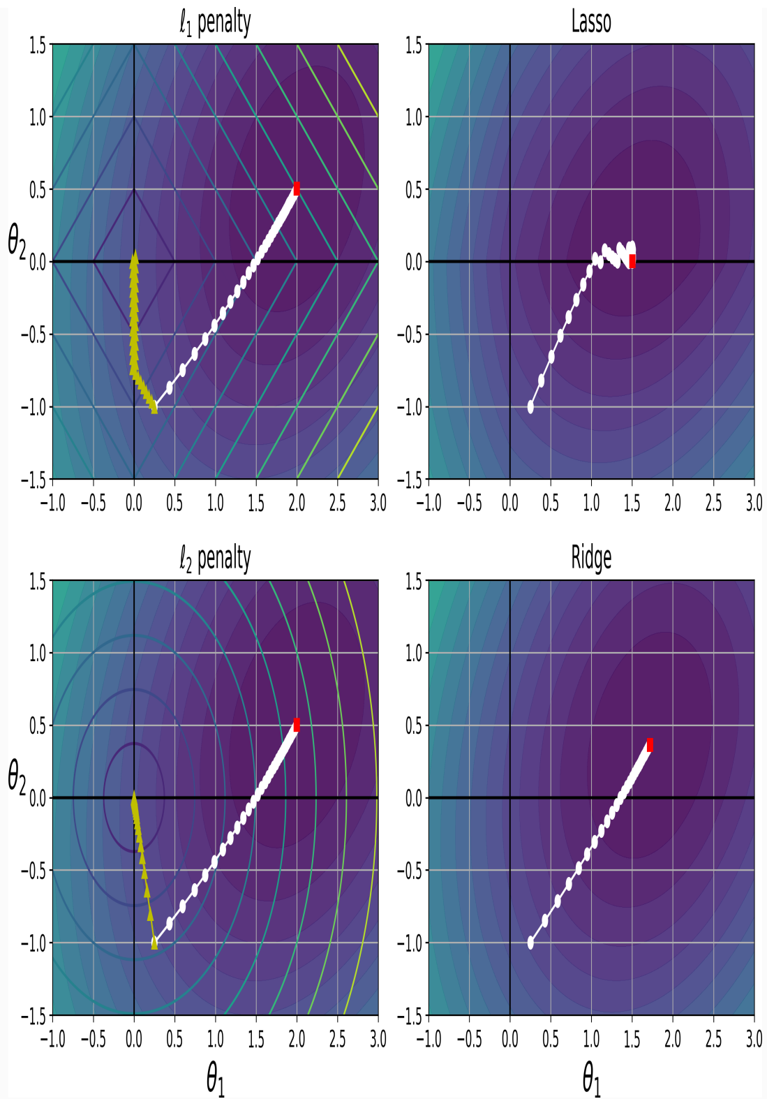
Figure 4-19. Lasso versus Ridge regularization
