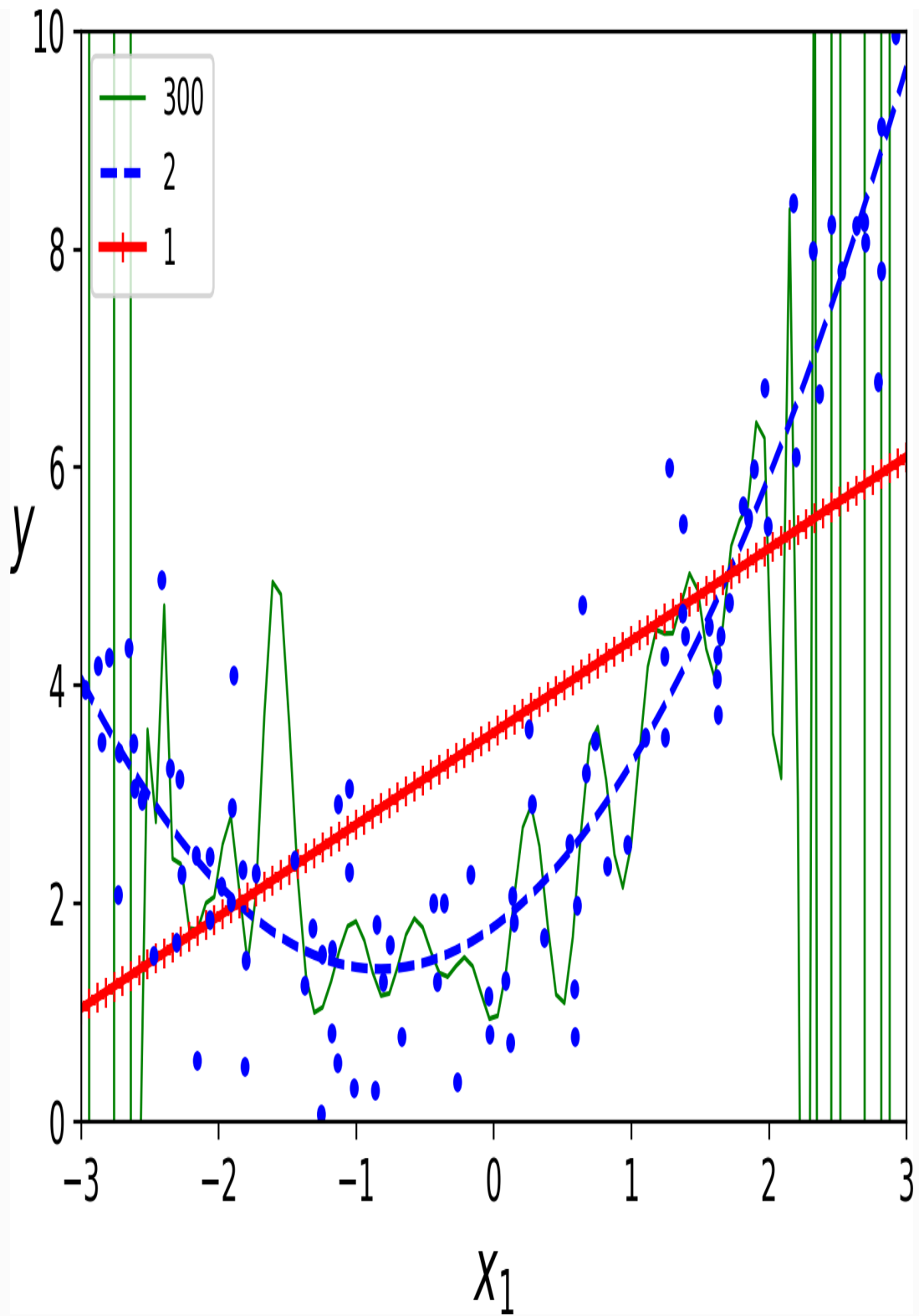
Figure 4-14. High-degree Polynomial Regression
