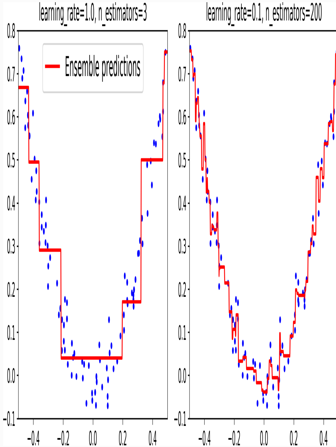
Figure 7-10. GBRT ensembles with not enough predictors (left) and too many (right)
