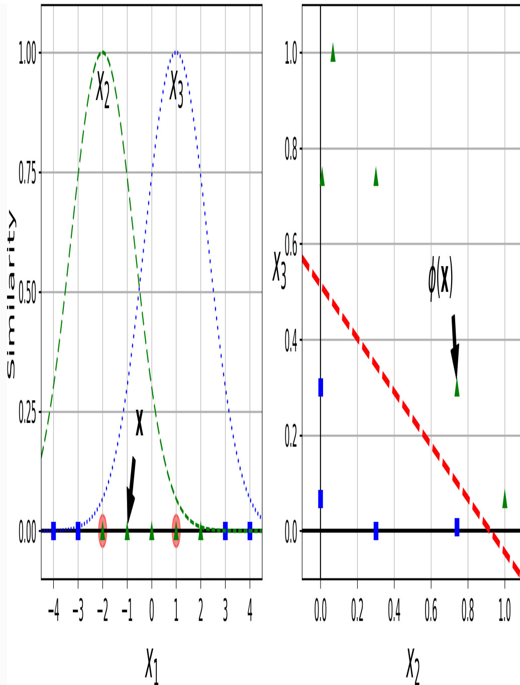
Figure 5-8. Similarity features using the Gaussian RBF
