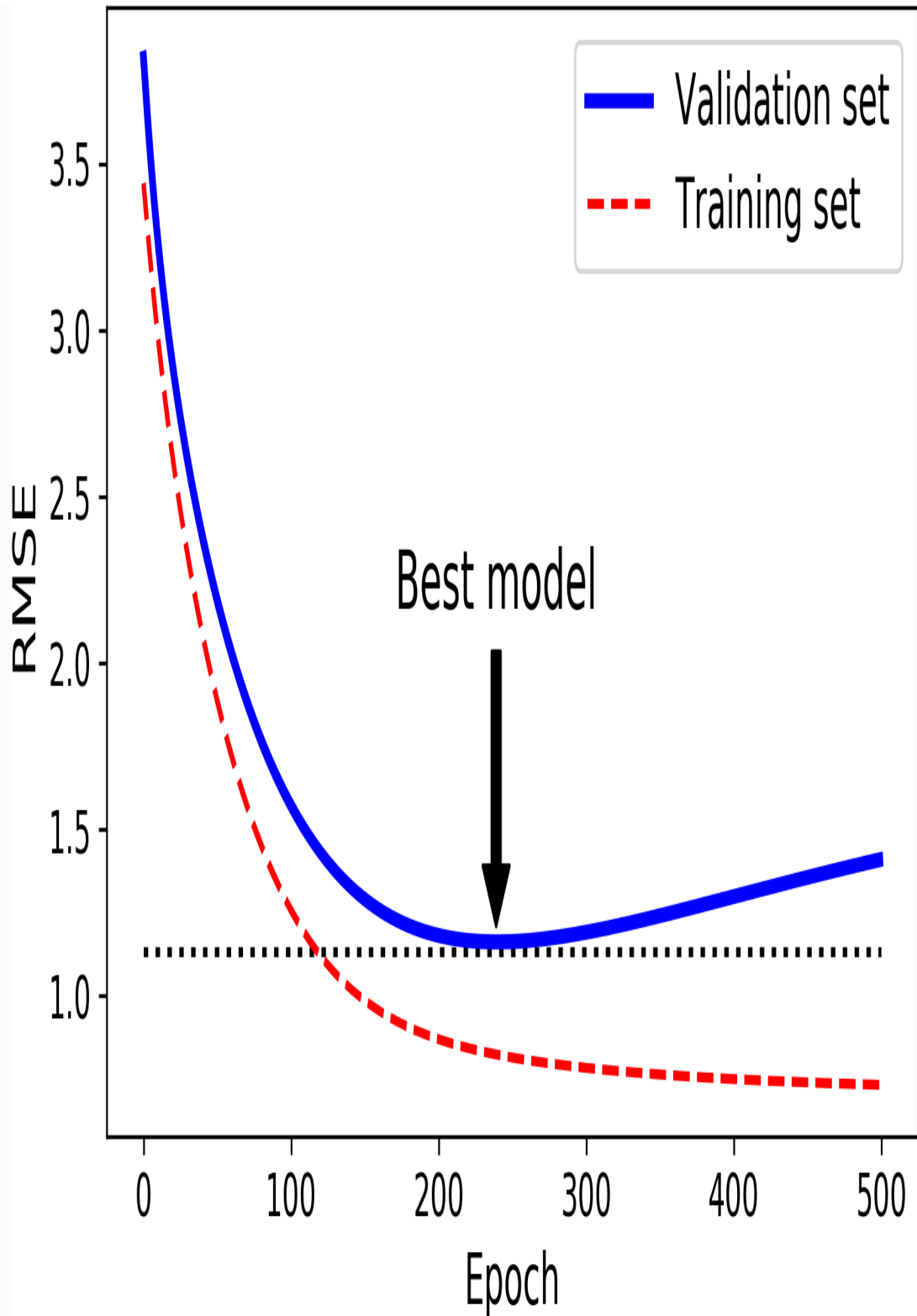
Figure 4-20. Early stopping regularization
