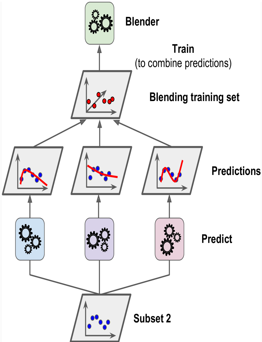
Figure 7-14. Training the blender
