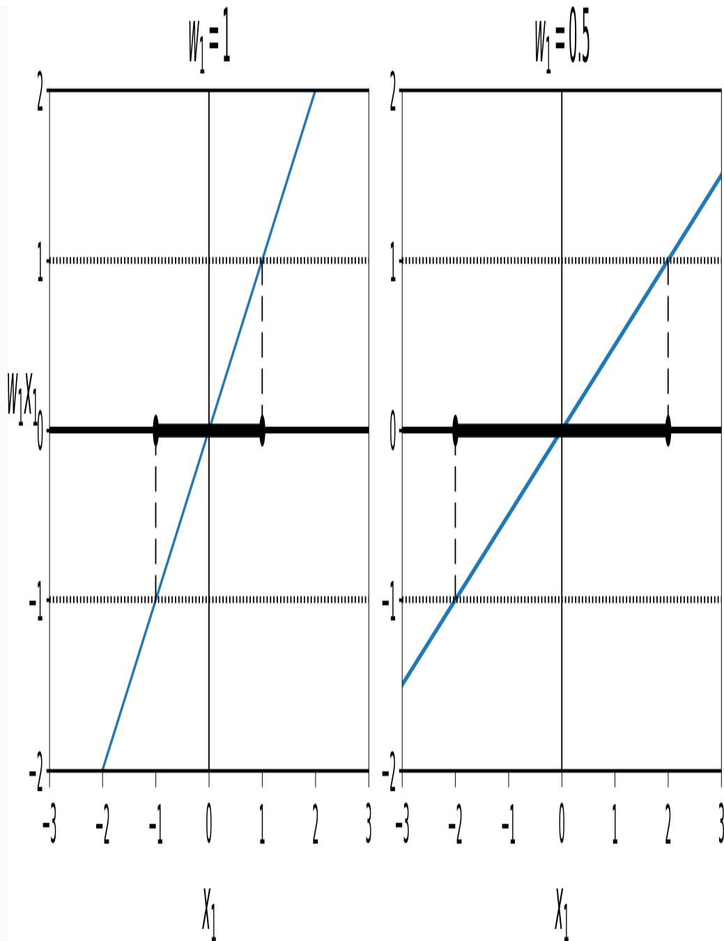
Figure 5-13. A smaller weight vector results in a larger margin
