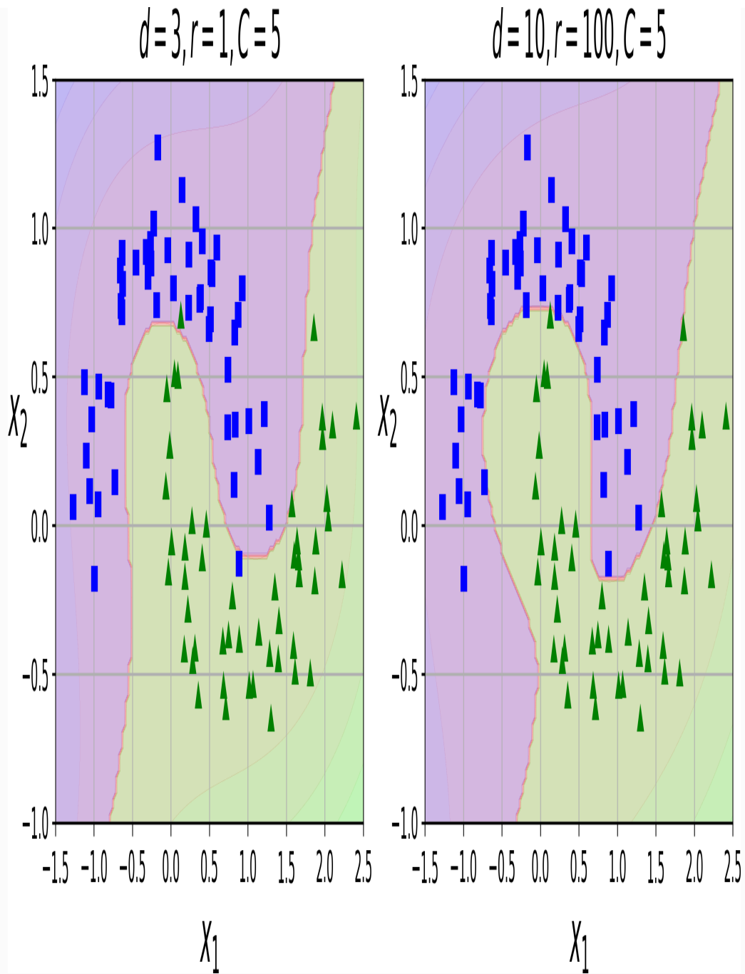
Figure 5-7. SVM classifiers with a polynomial kernel
