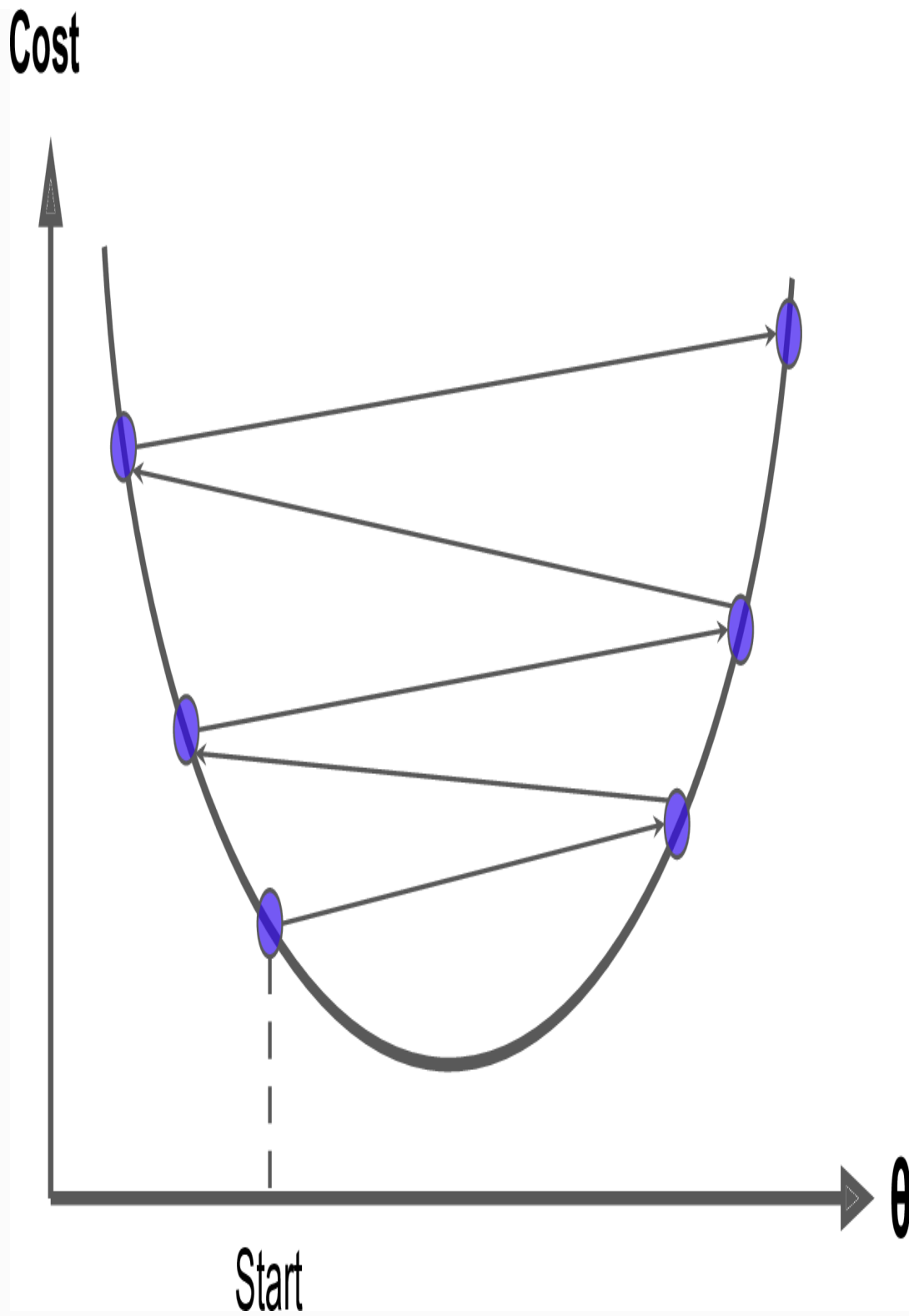
Figure 4-5. Learning rate too large
