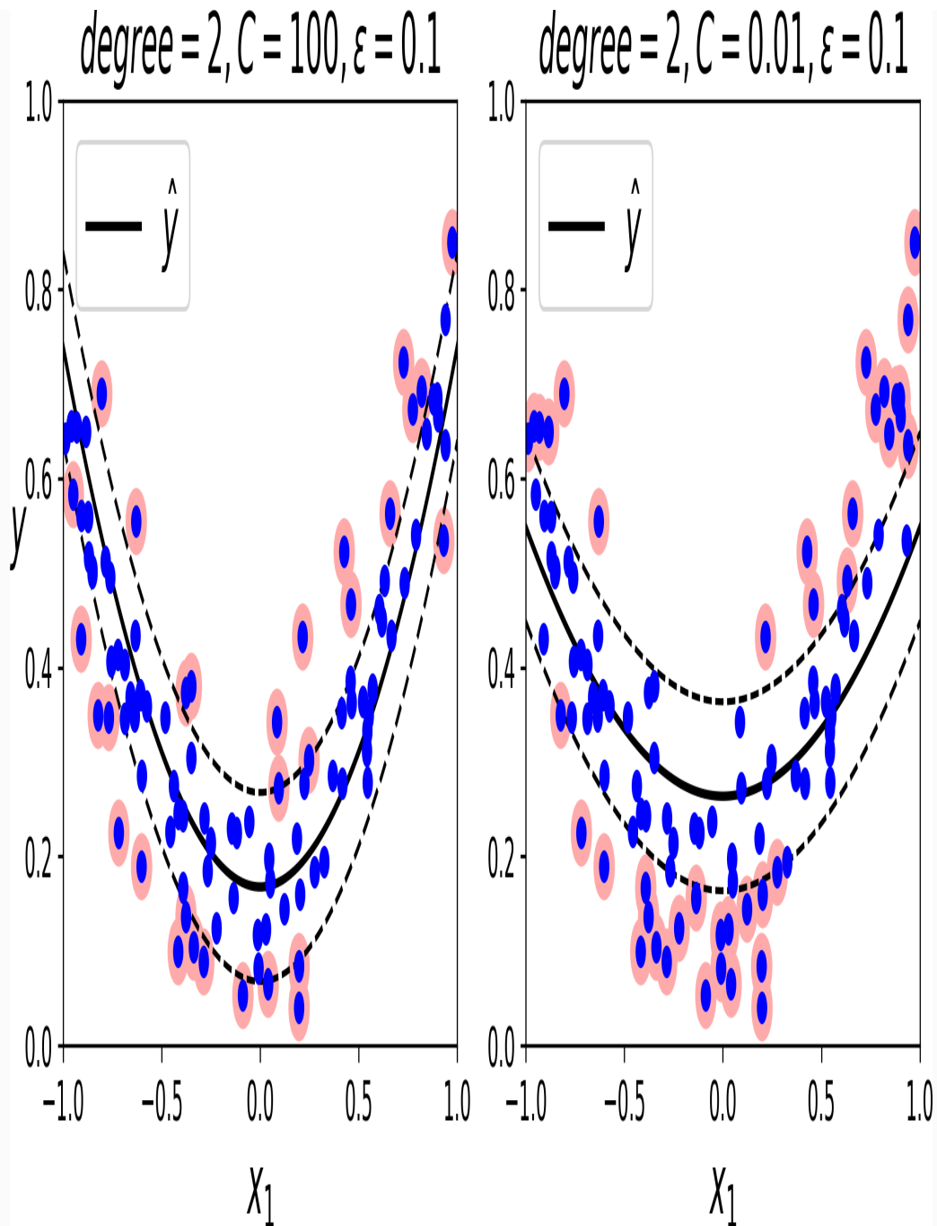
Figure 5-11. SVM regression using a 2 nd -degree polynomial kernel
