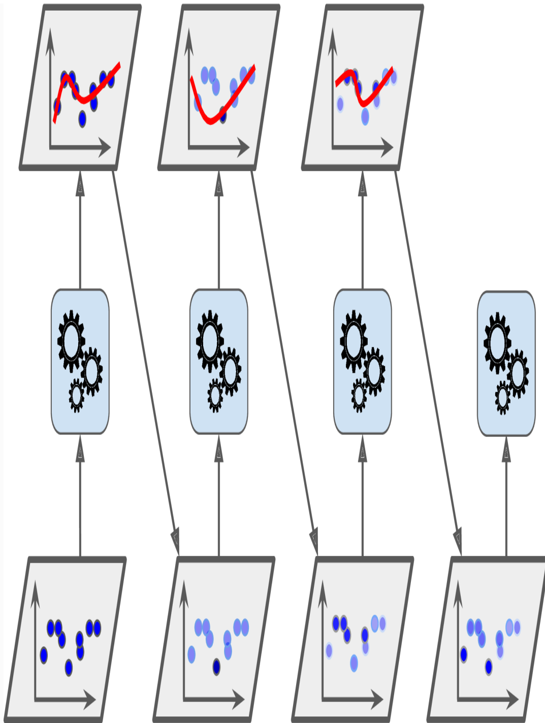
Figure 7-7. AdaBoost sequential training with instance weight updates
