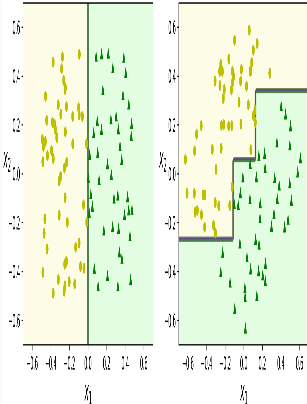
Figure 6-7. Sensitivity to training set rotation
