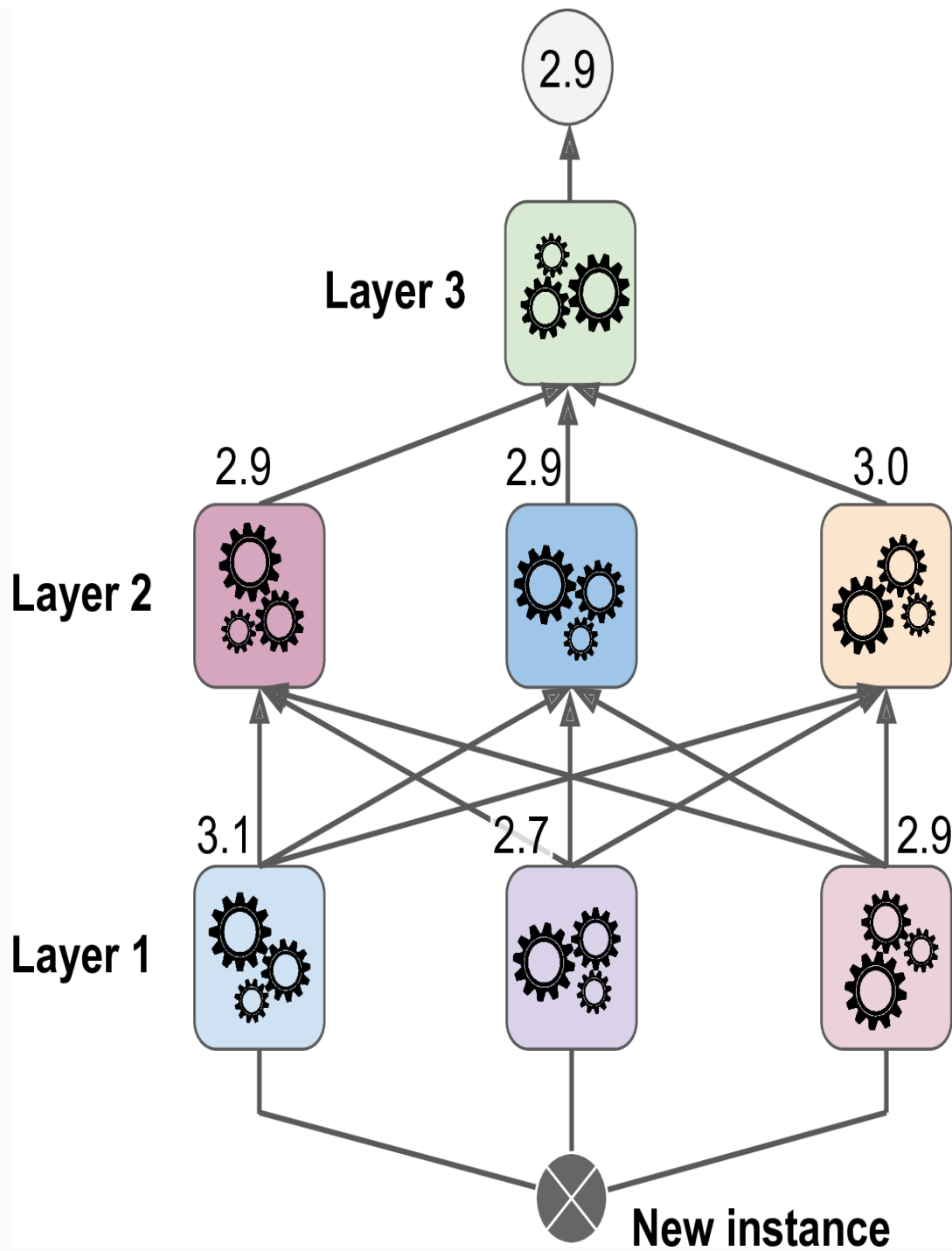
Figure 7-15. Predictions in a multilayer stacking ensemble
