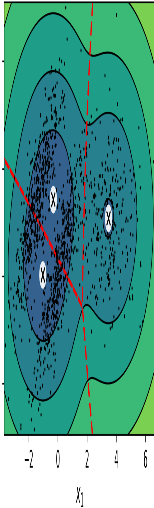
covariance_type="spherical"
