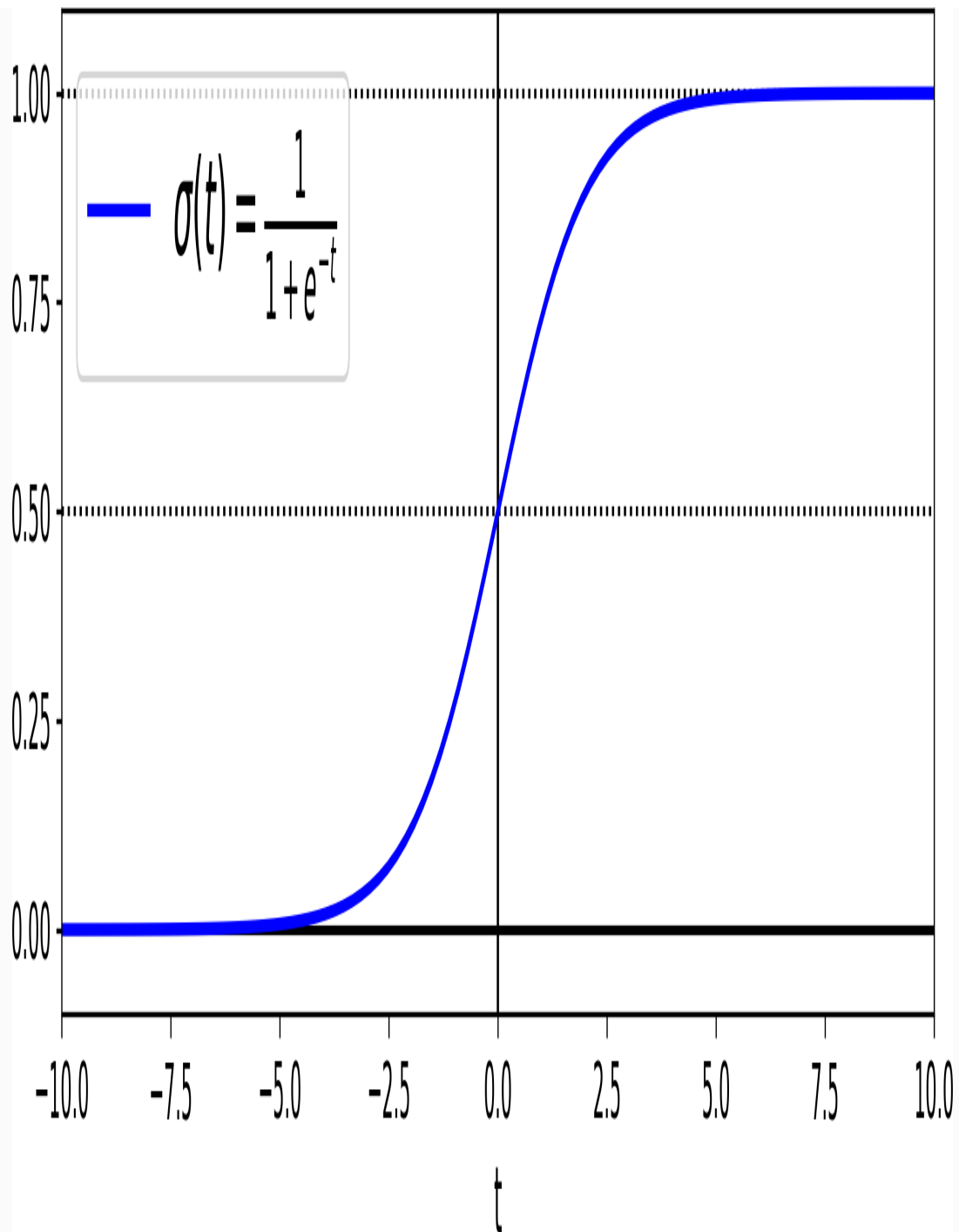
Figure 4-21. Logistic function
