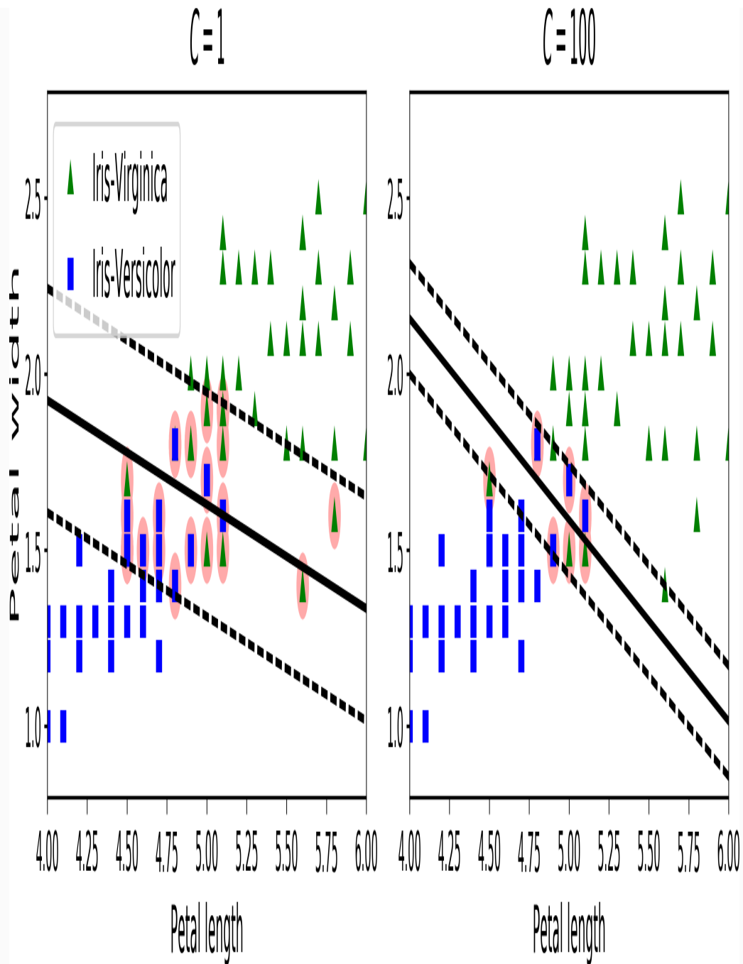
Figure 5-4. Large margin (left) versus fewer margin violations (right)
