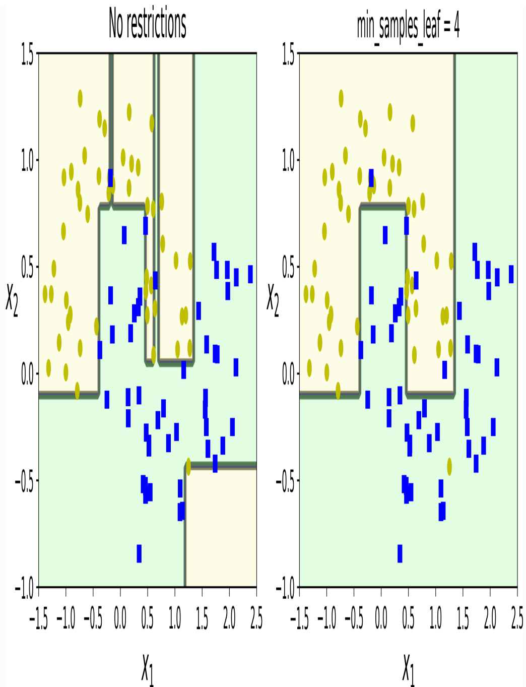
Figure 6-3. Regularization using min_samples_leaf
