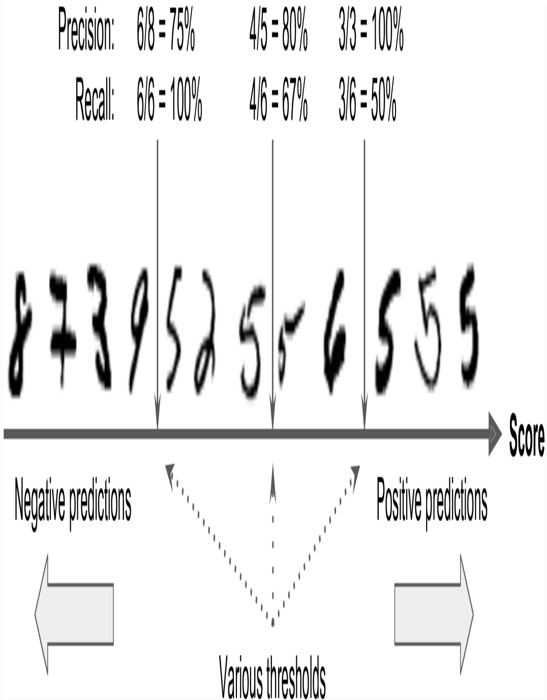
Figure 3-3. Decision threshold and precision/recall tradeoff
