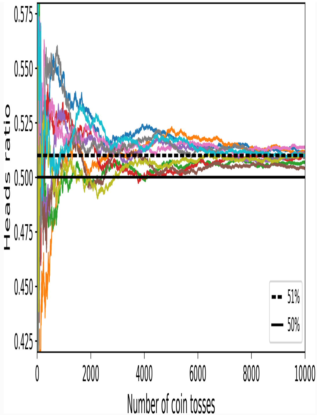
Figure 7-3. The law of large numbers
