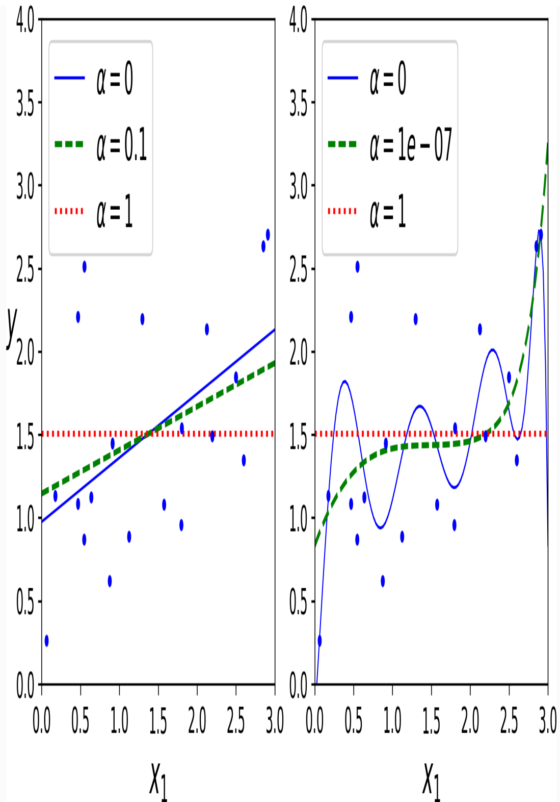
Figure 4-18. Lasso Regression
