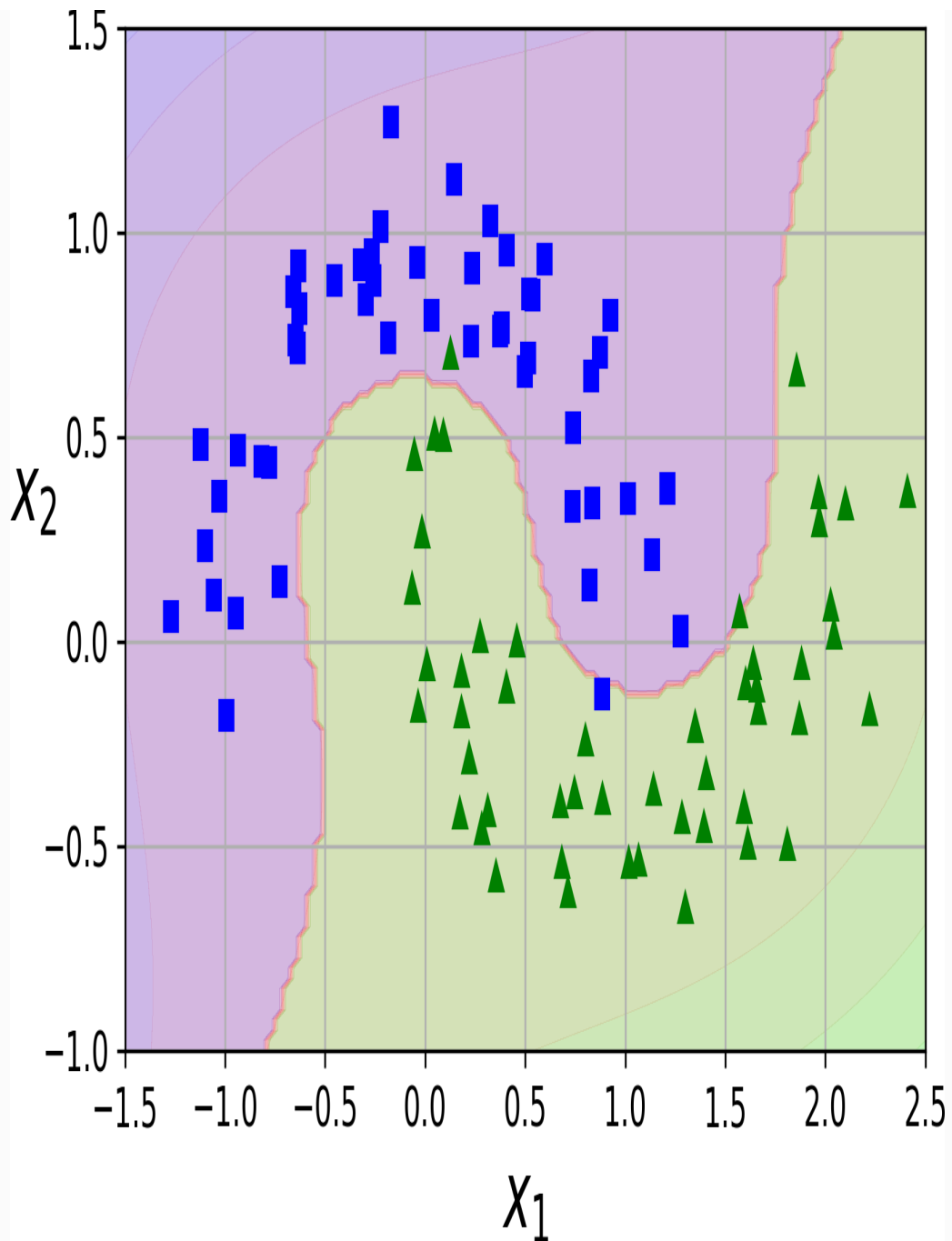
Figure 5-6. Linear SVM classifier using polynomial features
