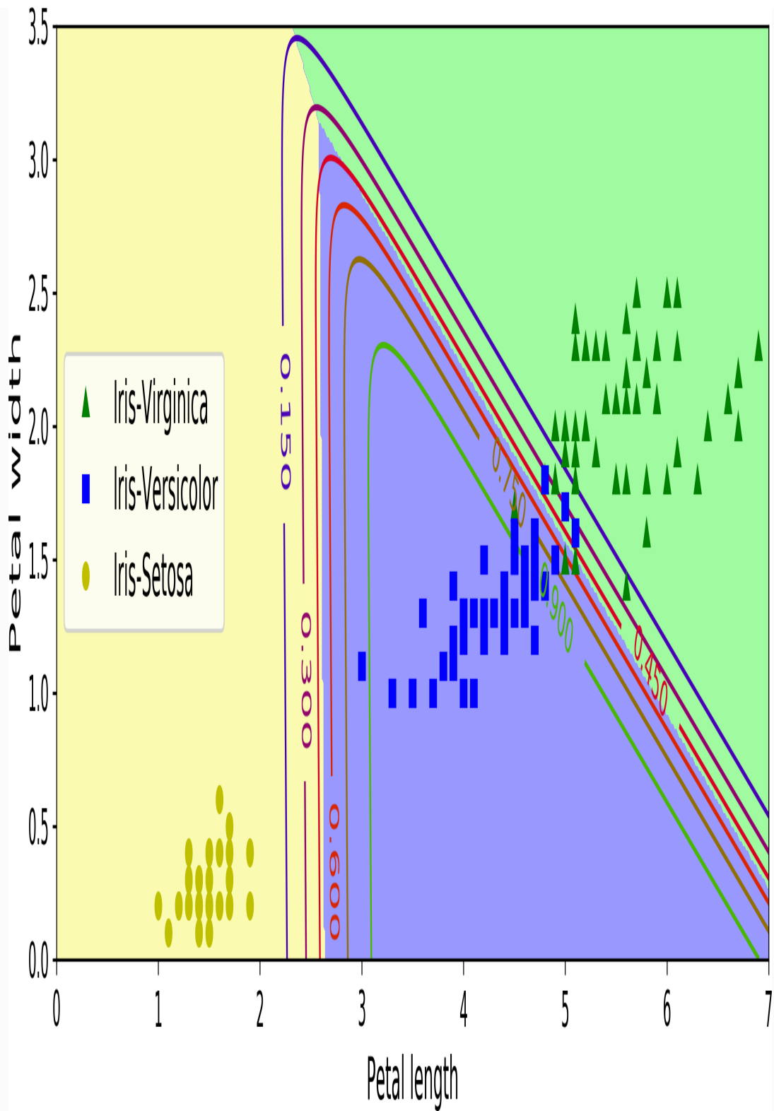
Figure 4-25. Softmax Regression decision boundaries
