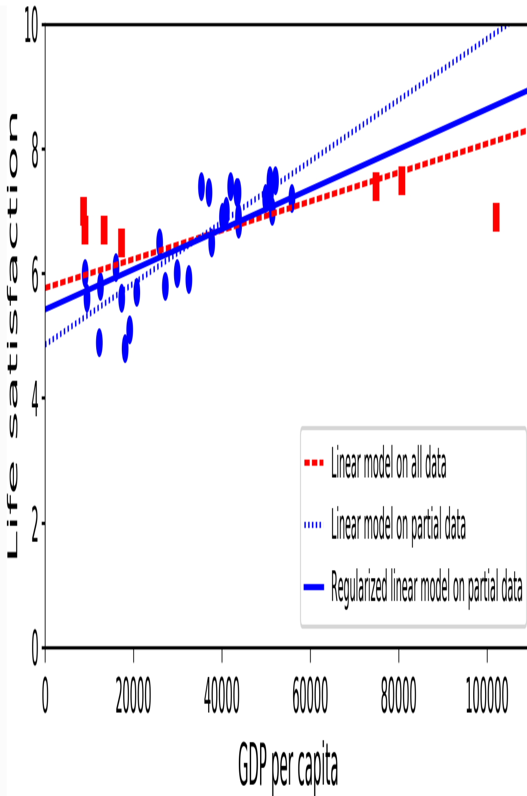
Figure 1-23. Regularization reduces the risk of overfitting
