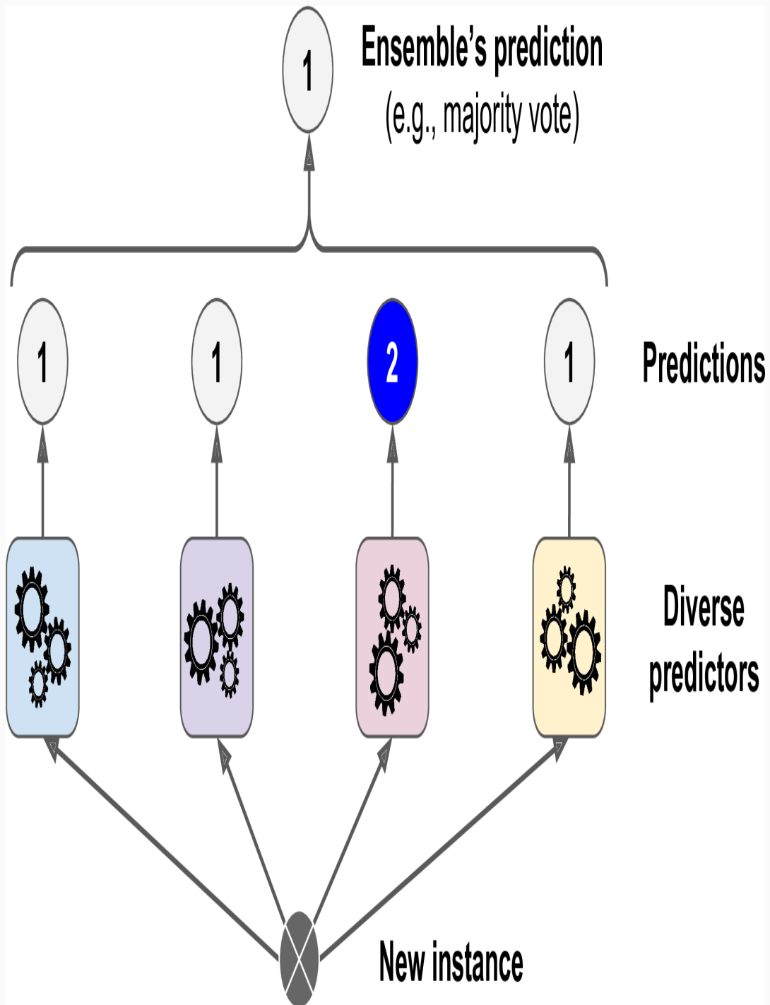
Figure 7-2. Hard voting classifier predictions
