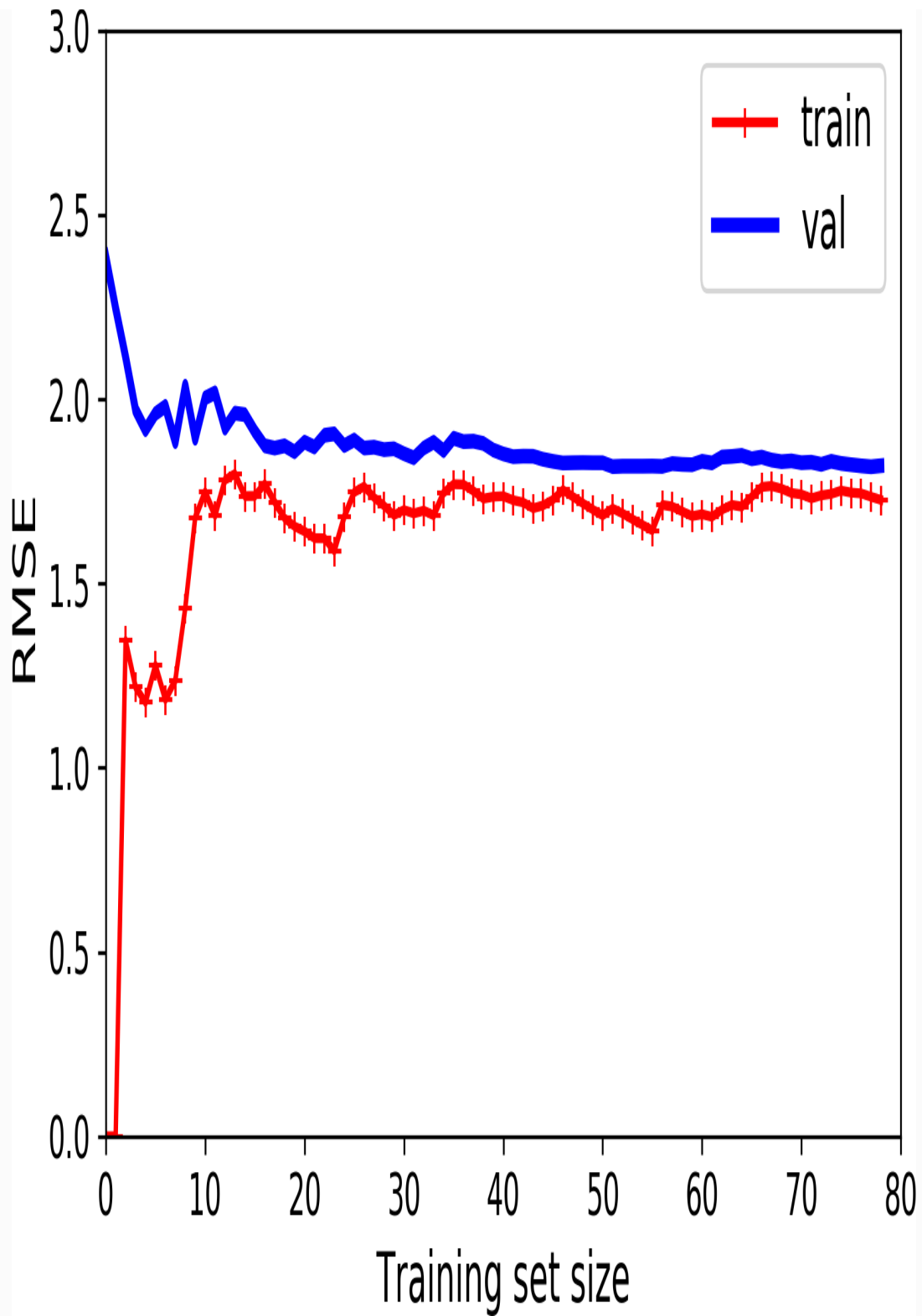
Figure 4-15. Learning curves
