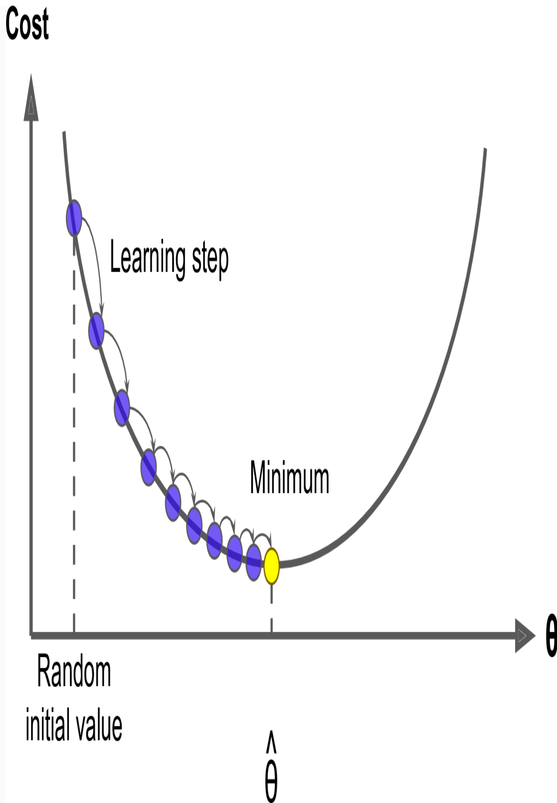
Figure 4-3. Gradient Descent
