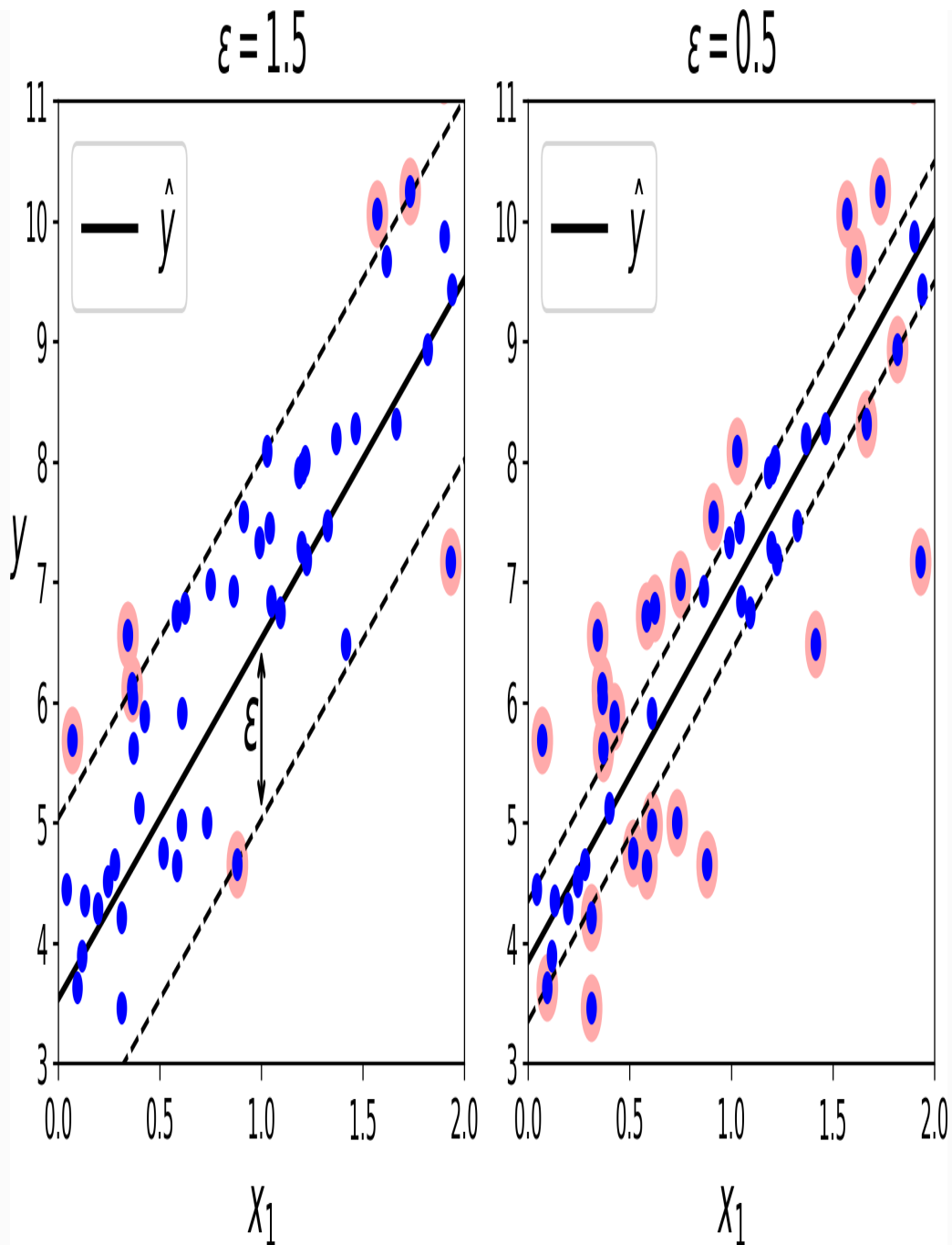
Figure 5-10. SVM Regression
