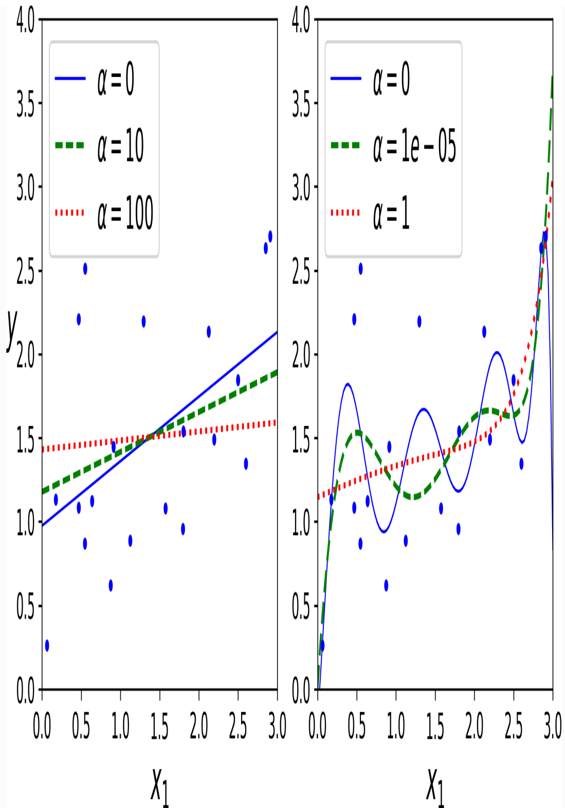
Figure 4-17. Ridge Regression
