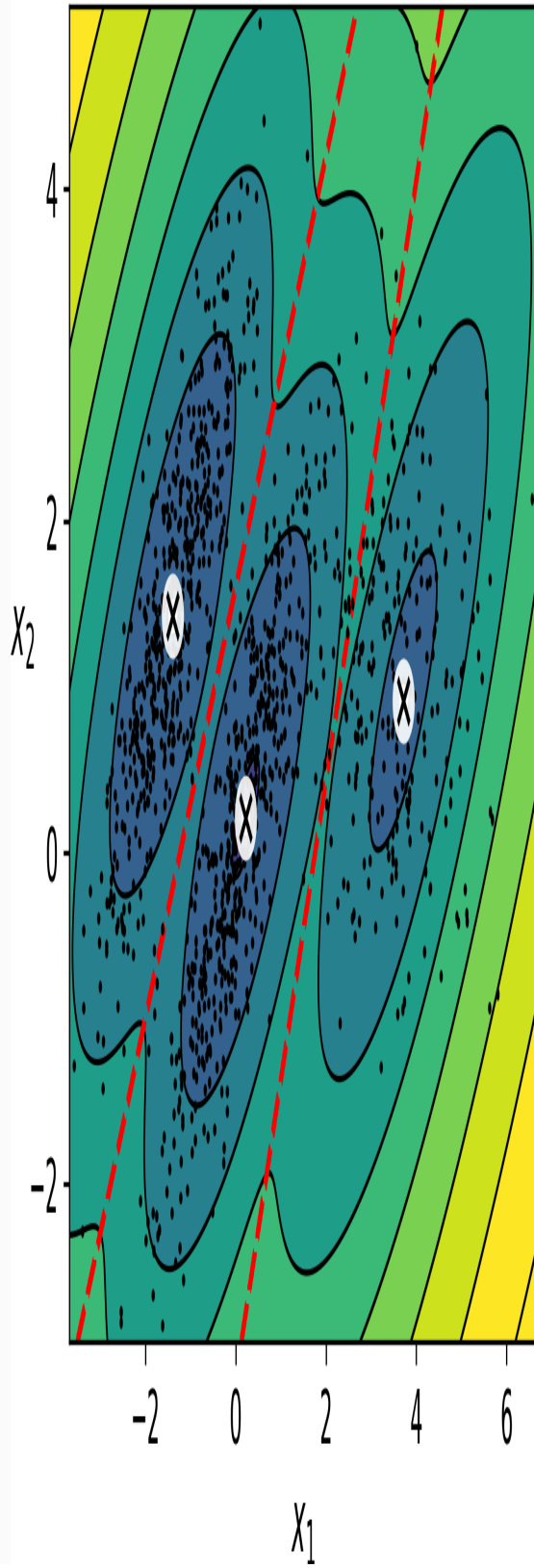
covariance_type="tied"
