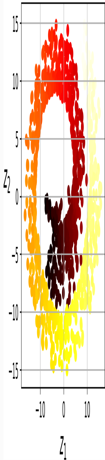
MDS
