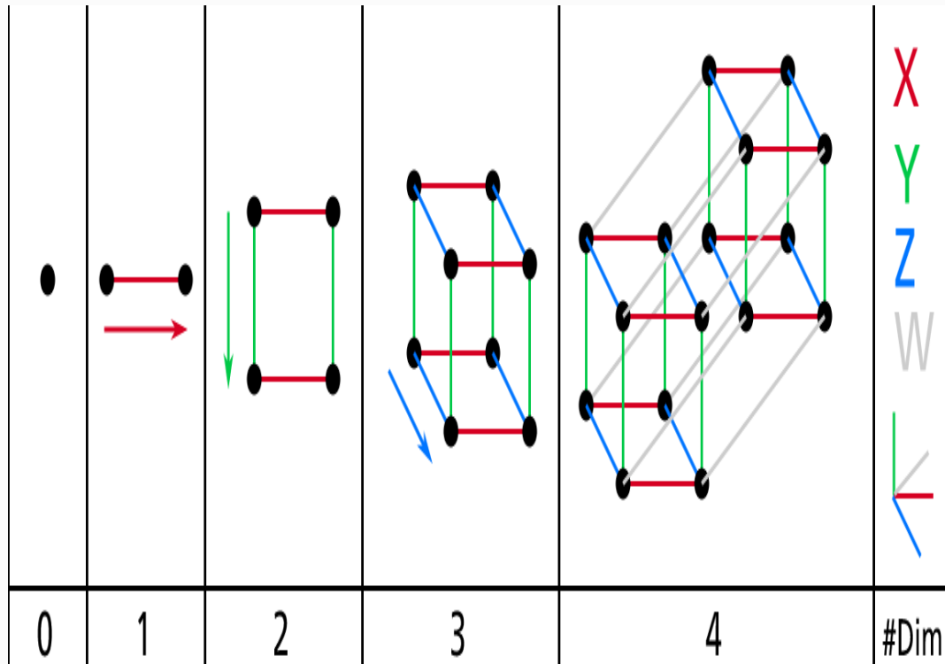
Figure 8-1. Point, segment, square, cube, and tesseract (0D to 4D hypercubes) 2
