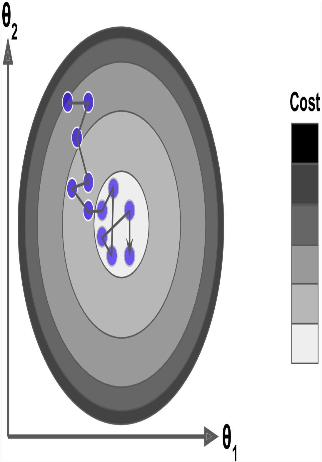
Figure 4-9. Stochastic Gradient Descent
