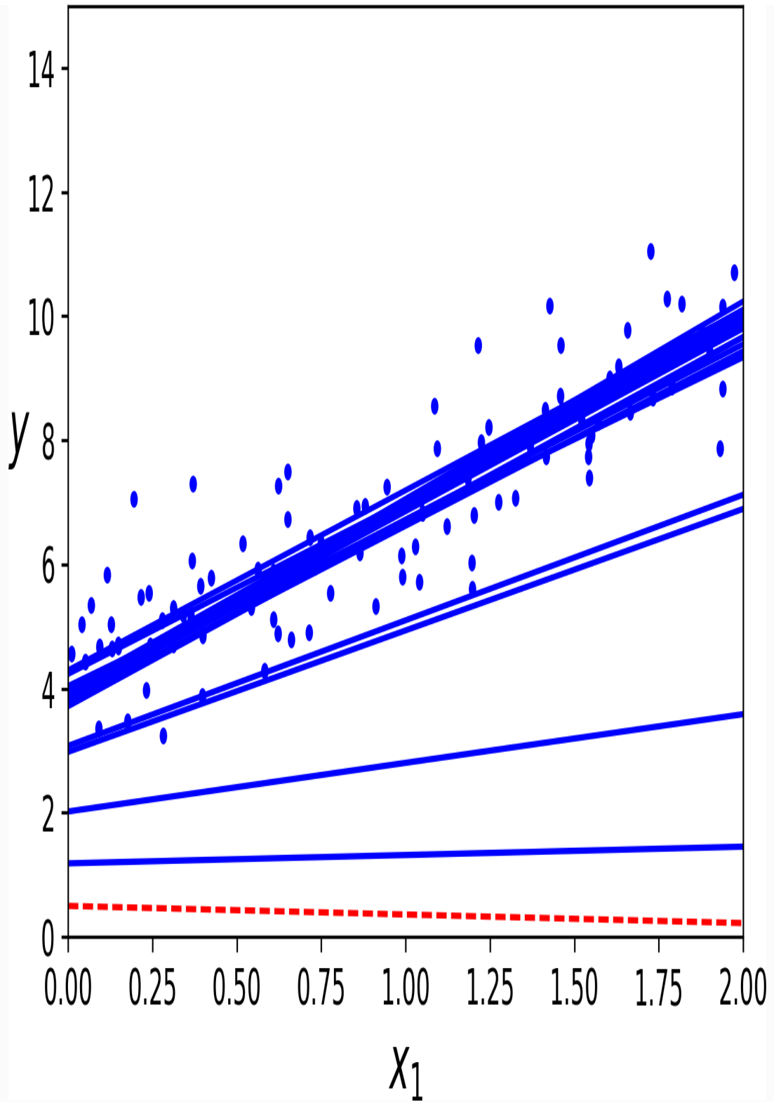
Figure 4-10. Stochastic Gradient Descent first 20 steps
