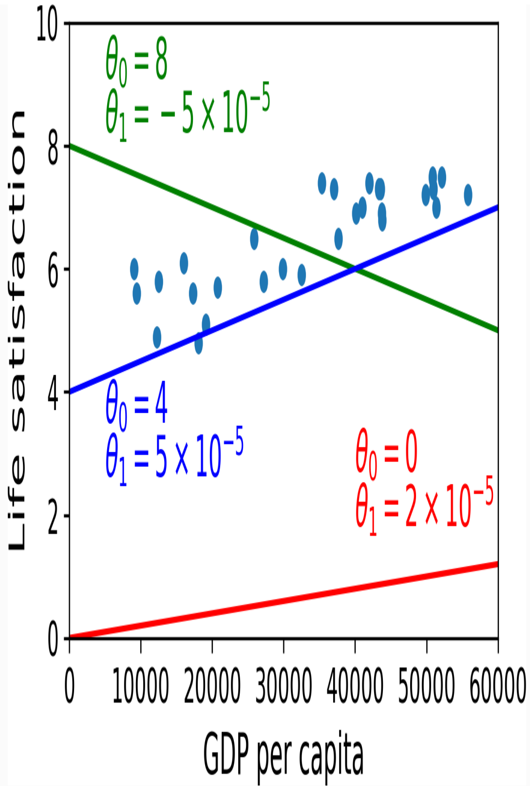
Figure 1-18. A few possible linear models
