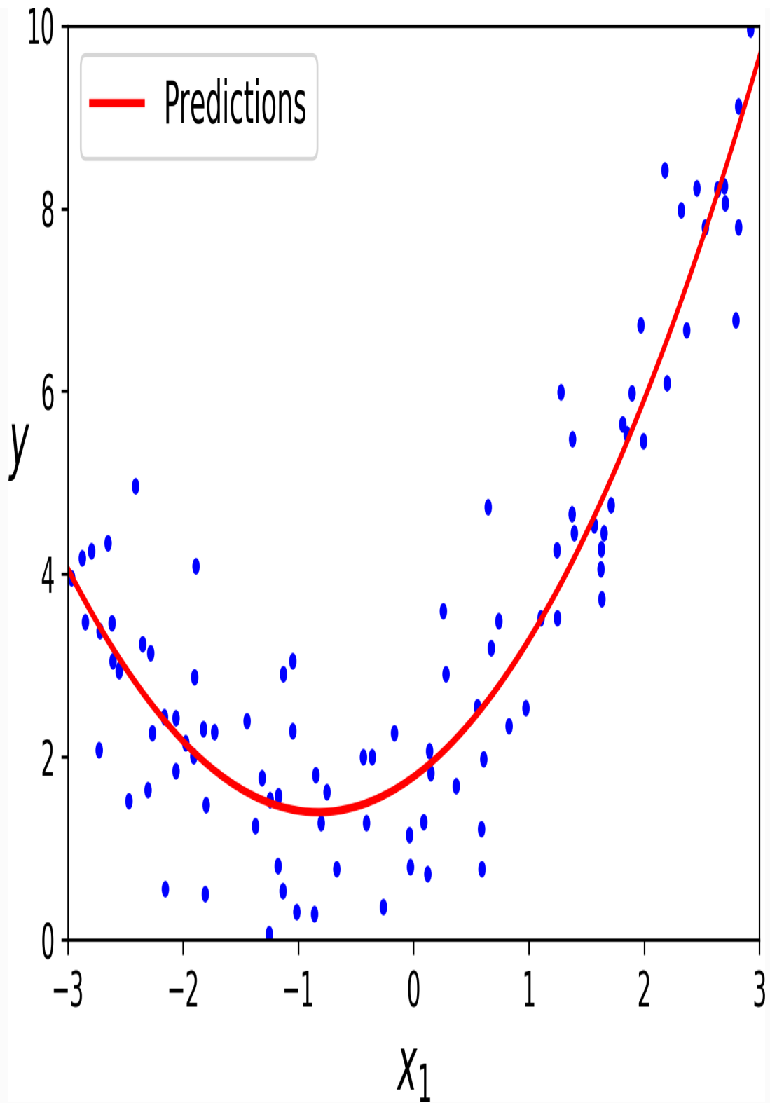
Figure 4-13. Polynomial Regression model predictions
