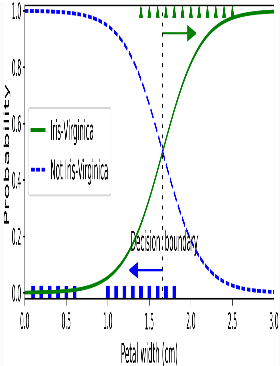
Figure 4-23. Estimated probabilities and decision boundary
