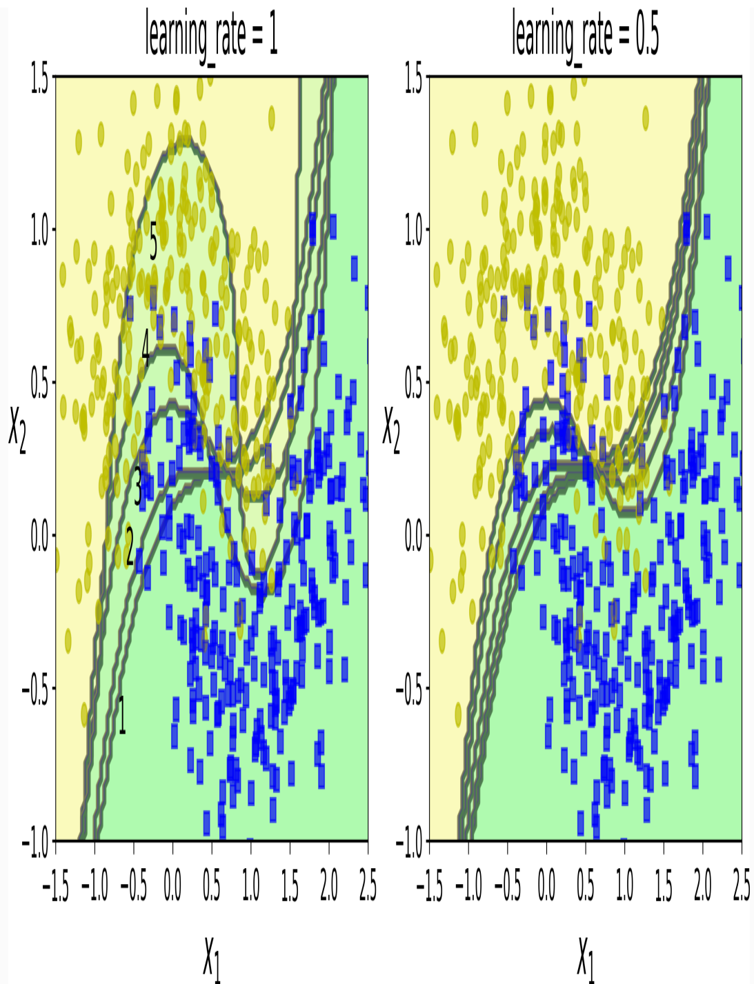
Figure 7-8. Decision boundaries of consecutive predictors
