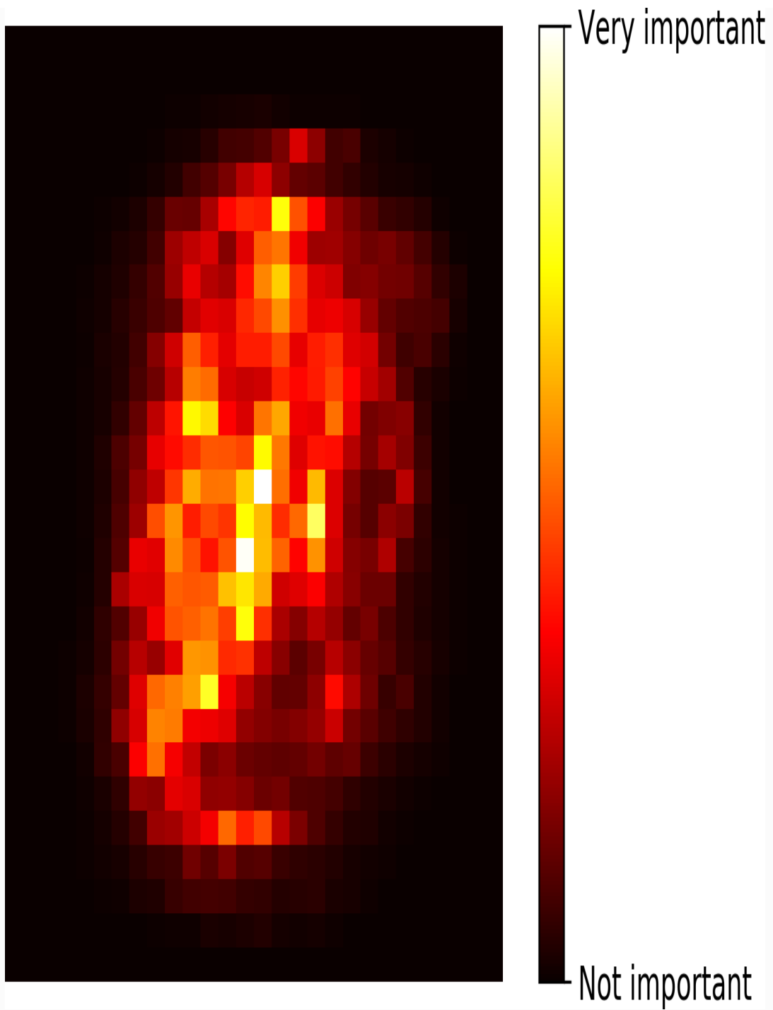
Figure 7-6. MNIST pixel importance (according to a Random Forest classifier)
