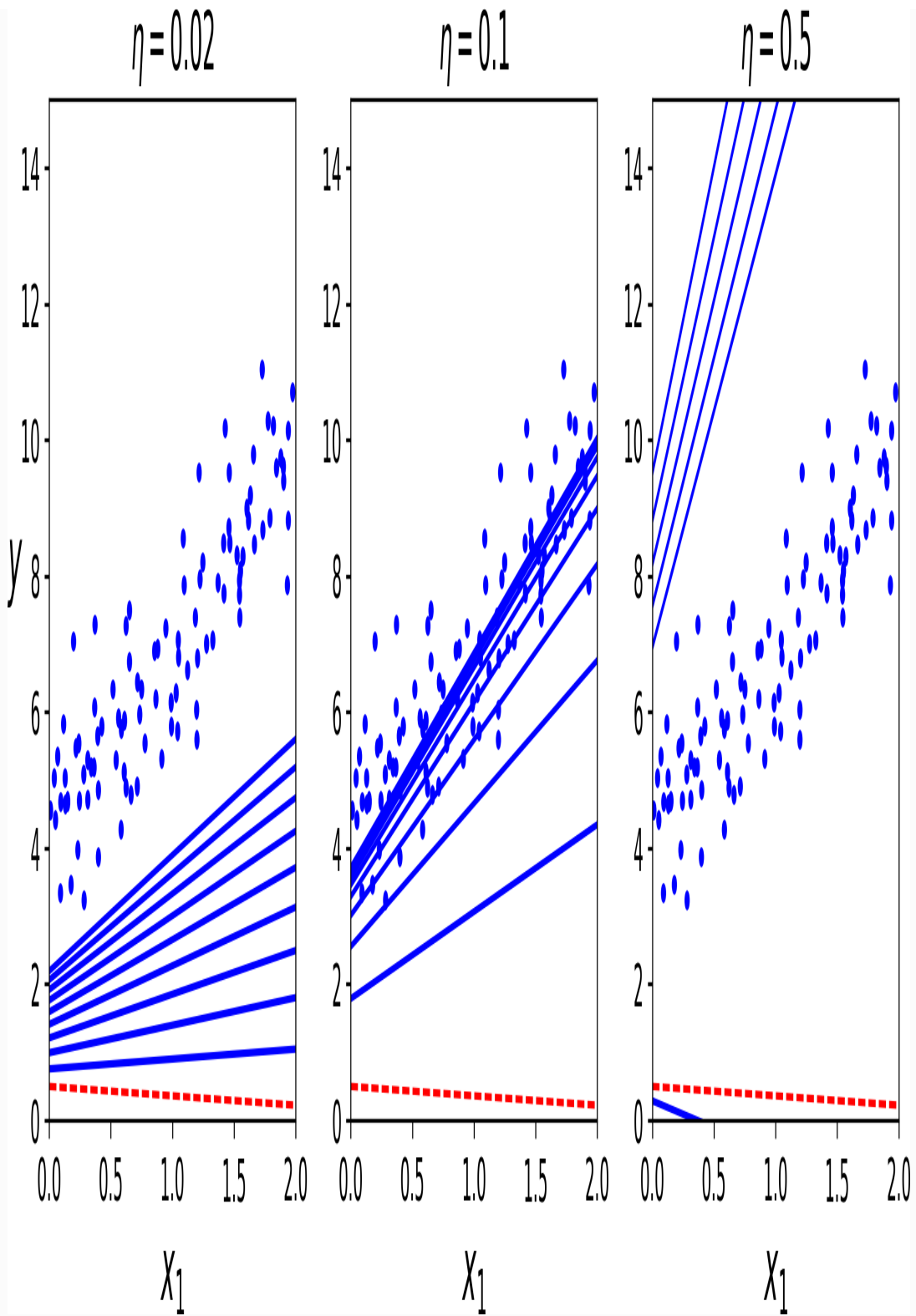
Figure 4-8. Gradient Descent with various learning rates
