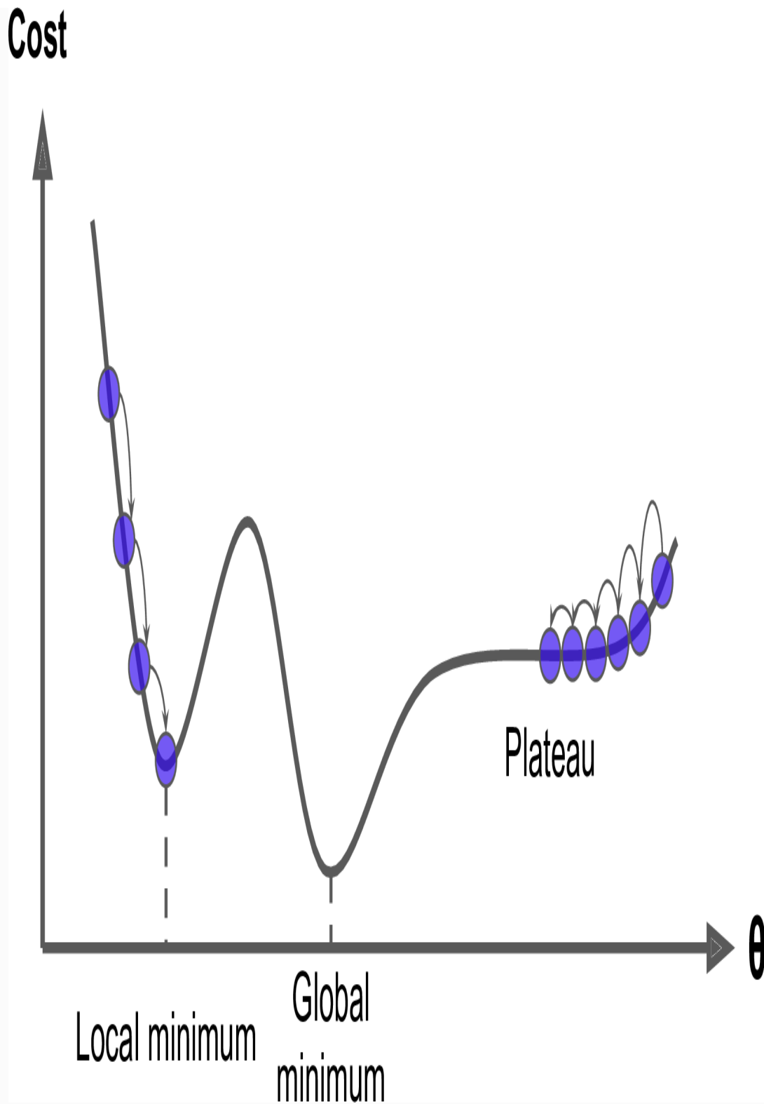
Figure 4-6. Gradient Descent pitfalls
