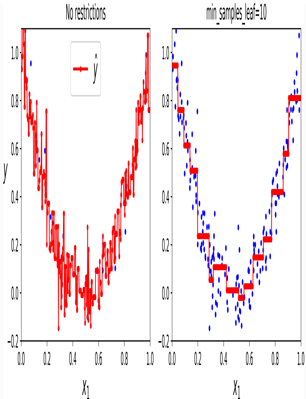
Figure 6-6. Regularizing a Decision Tree regressor
