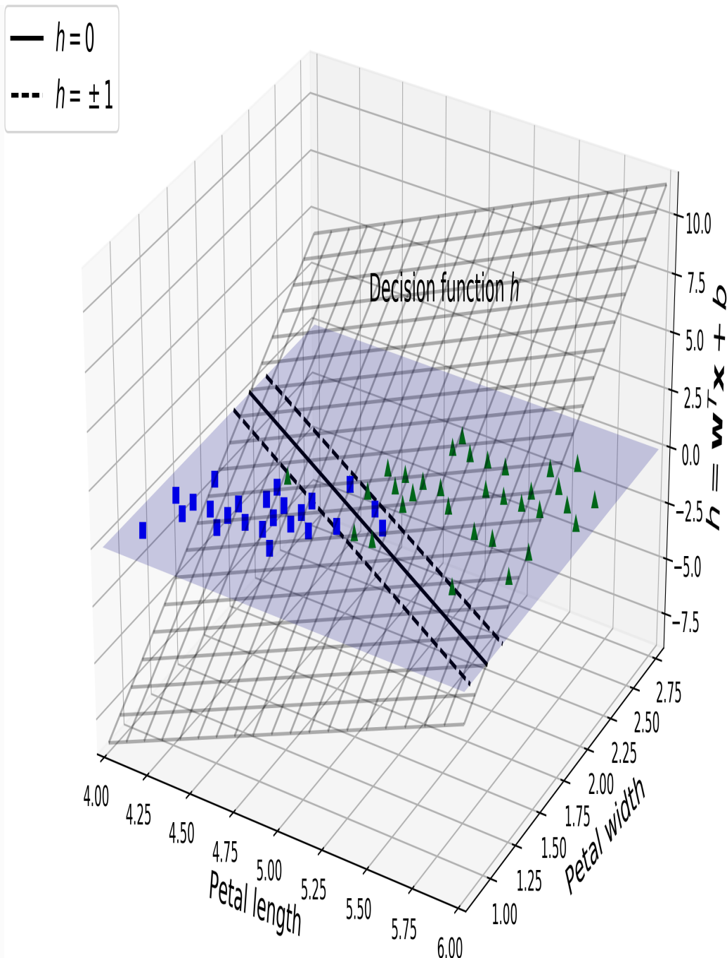
Figure 5-12. Decision function for the iris dataset
