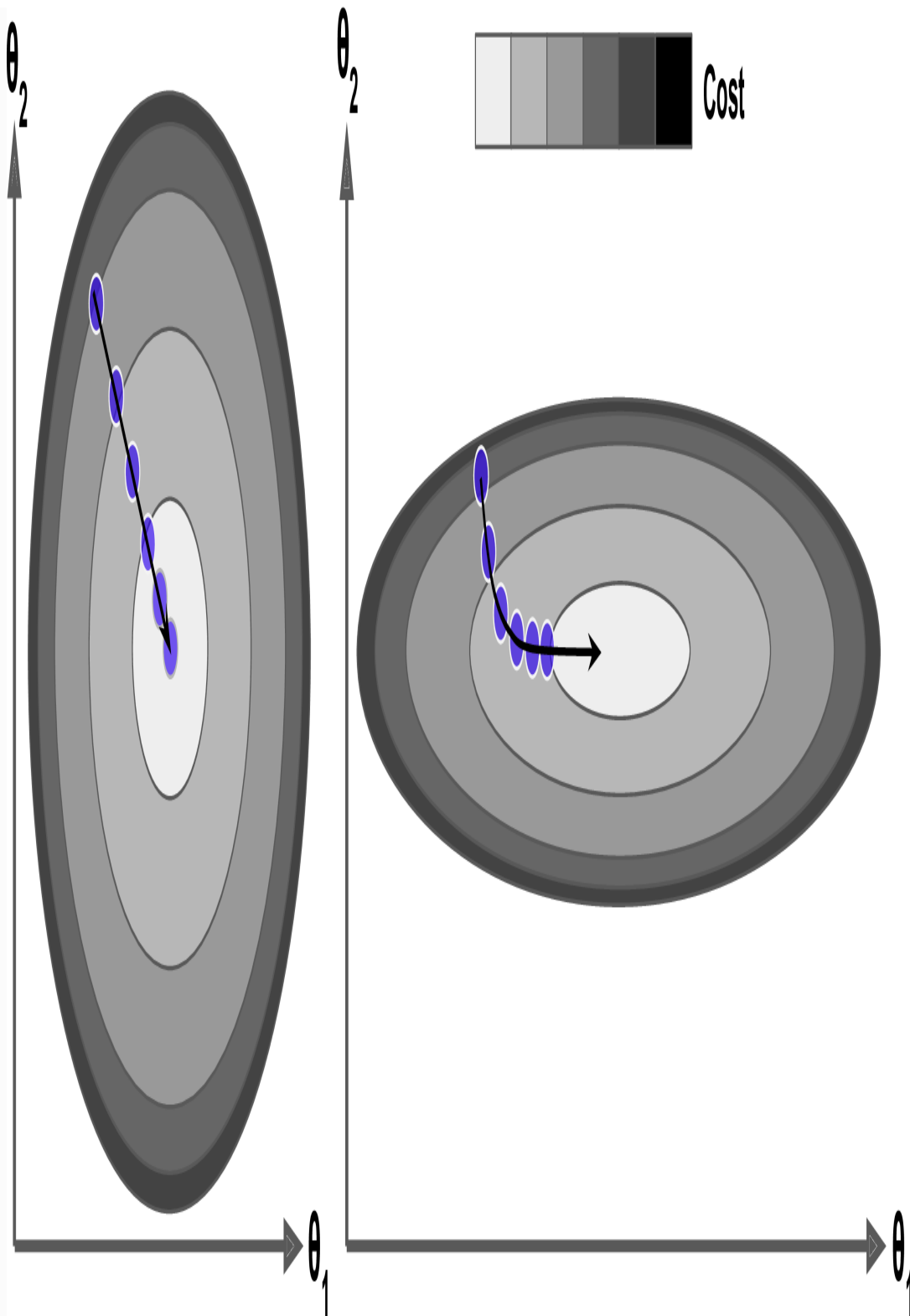
Figure 4-7. Gradient Descent with and without feature scaling
