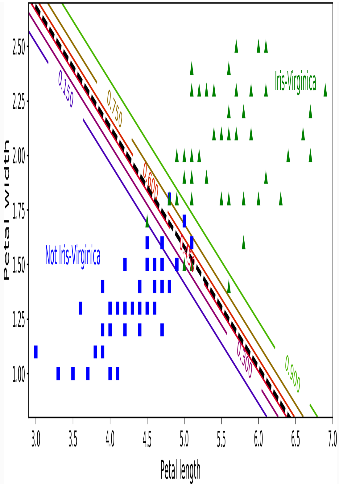
Figure 4-24. Linear decision boundary
