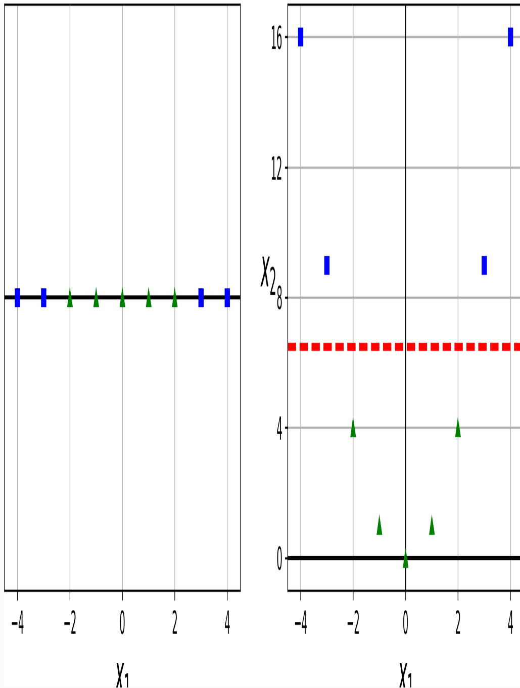
Figure 5-5. Adding features to make a dataset linearly separable
