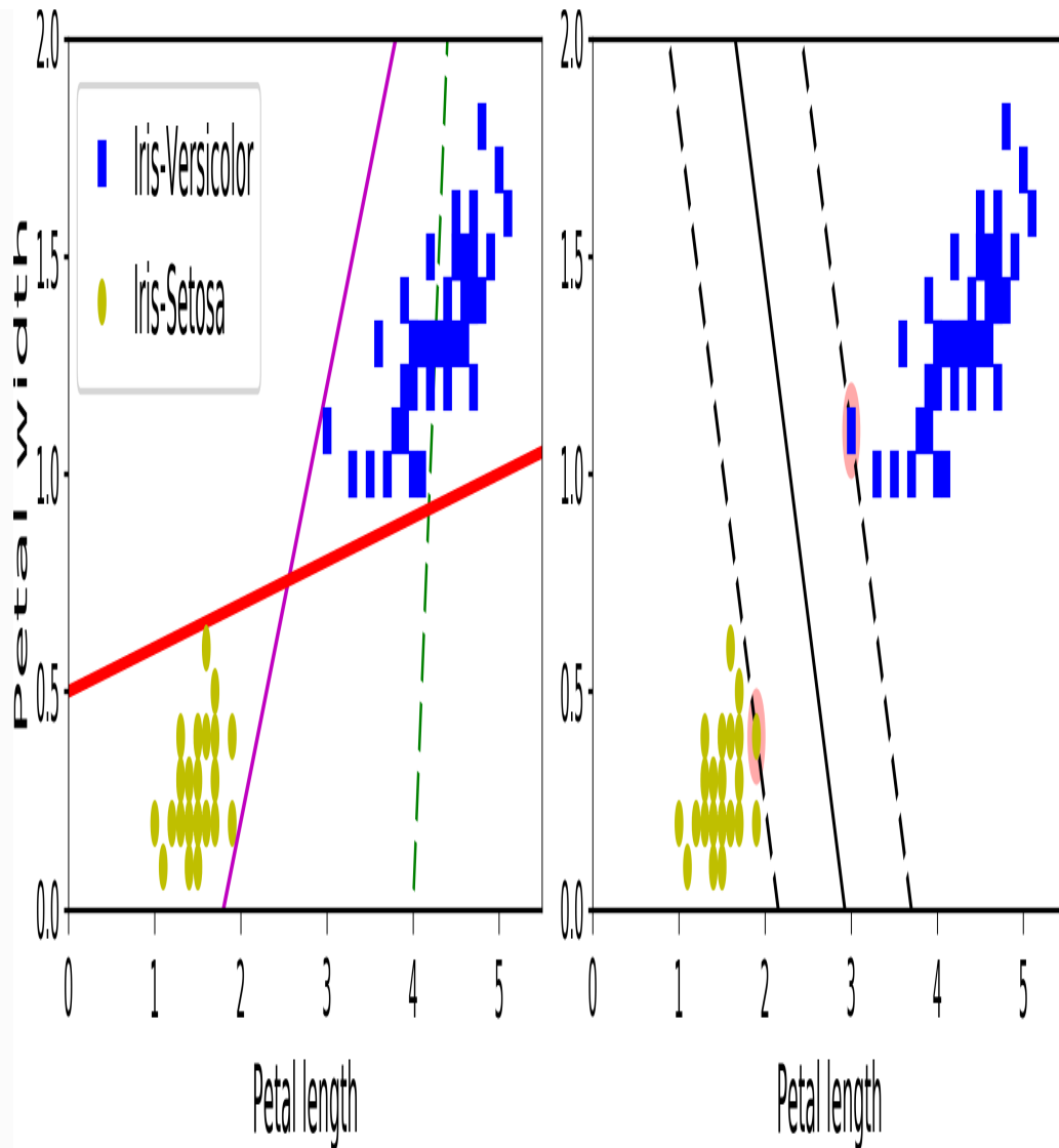
Figure 5-1. Large margin classification
