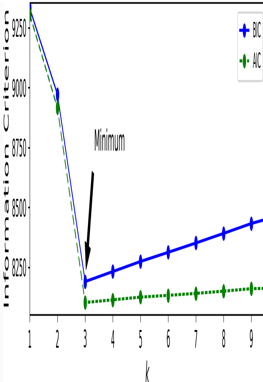
Figure 9-21. AIC and BIC for different numbers of clusters k
