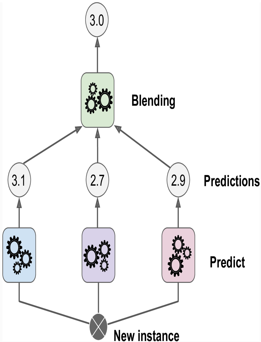
Figure 7-12. Aggregating predictions using a blending predictor
