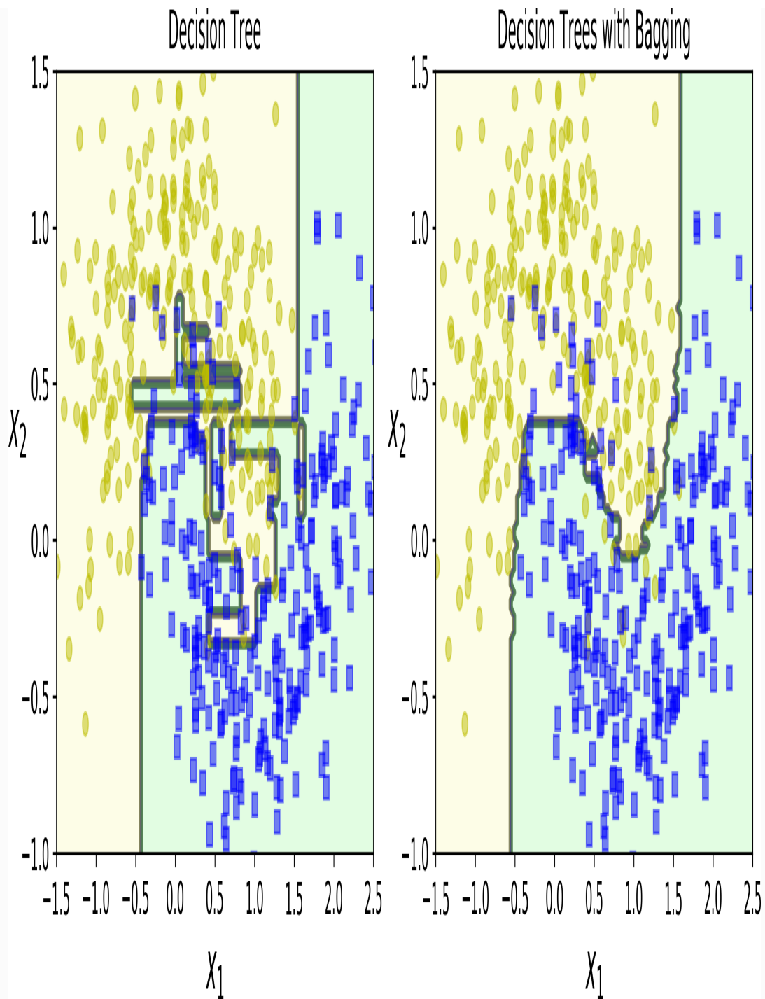
Figure 7-5. A single Decision Tree versus a bagging ensemble of 500 trees
