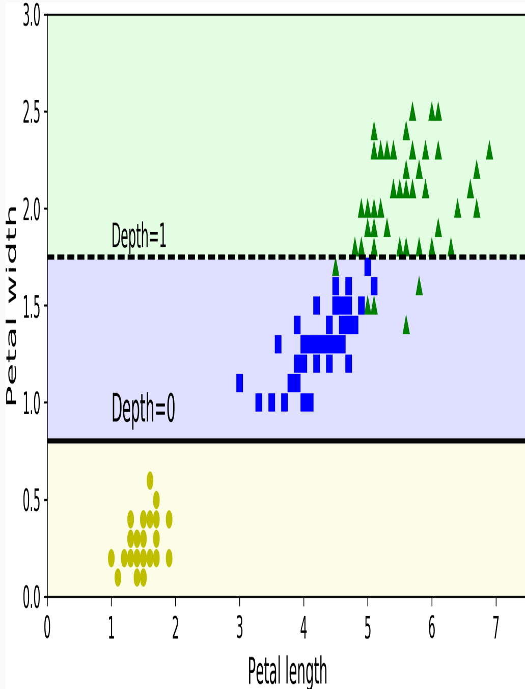
Figure 6-8. Sensitivity to training set details
