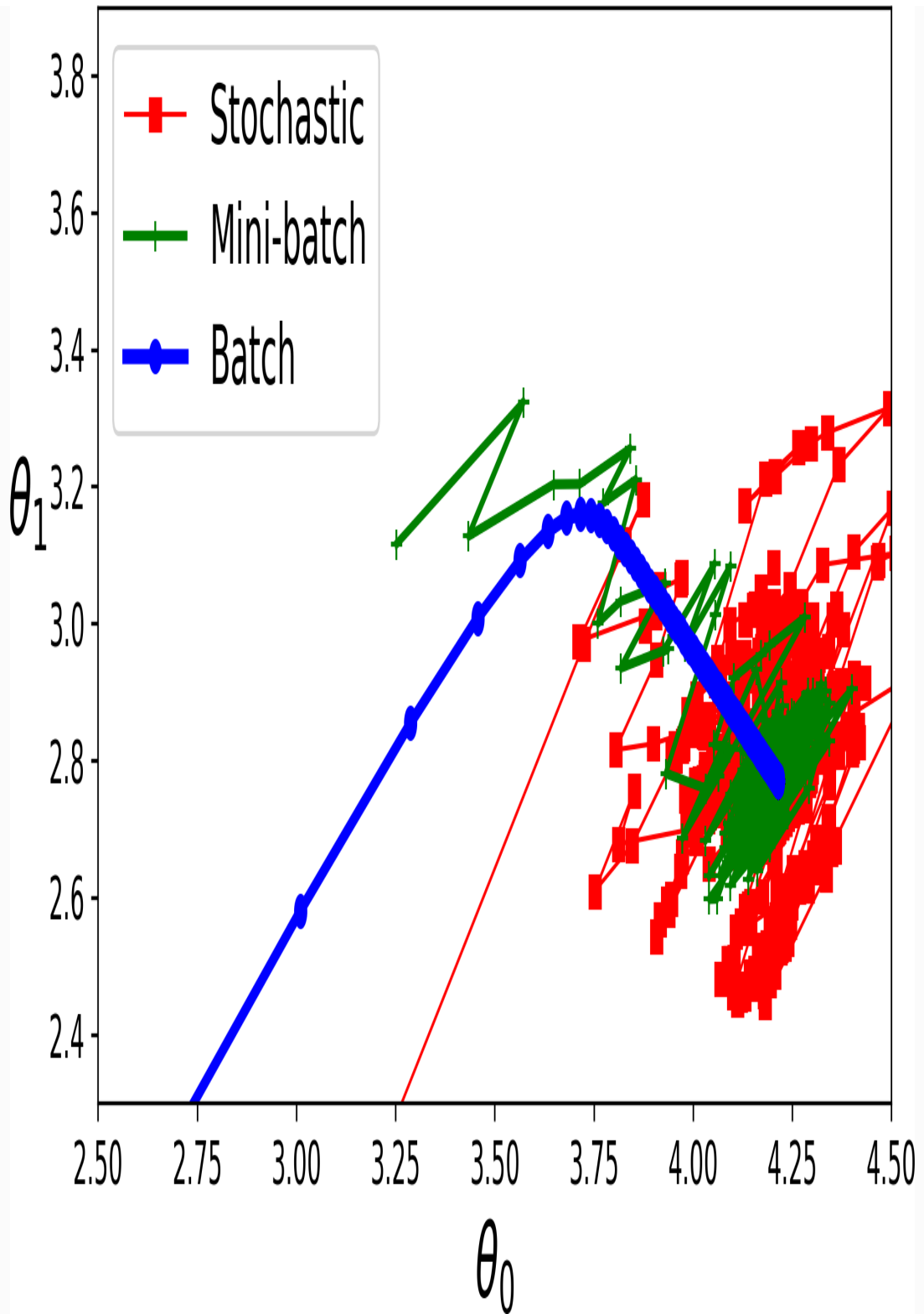
Figure 4-11. Gradient Descent paths in parameter space
