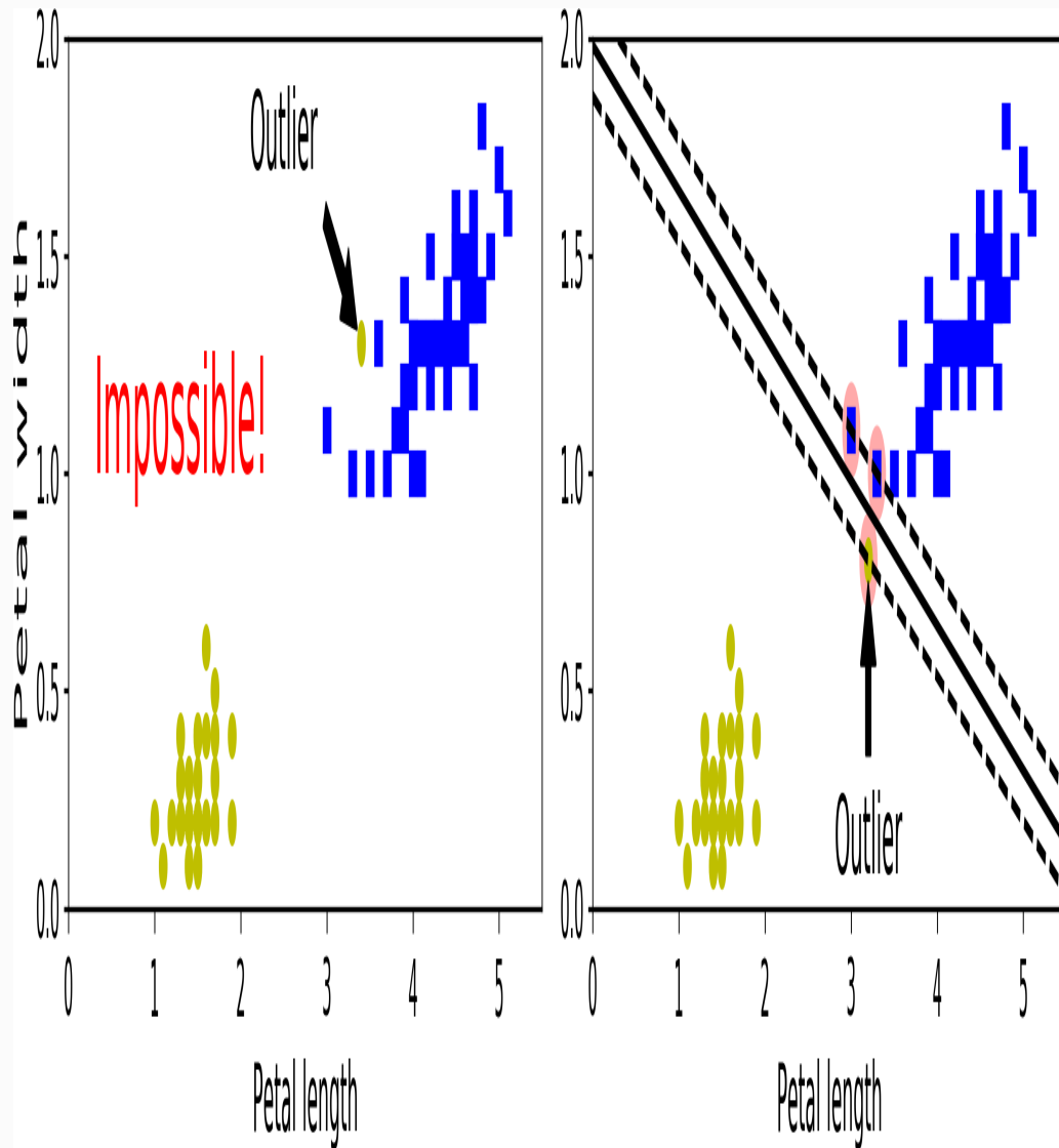
Figure 5-3. Hard margin sensitivity to outliers
