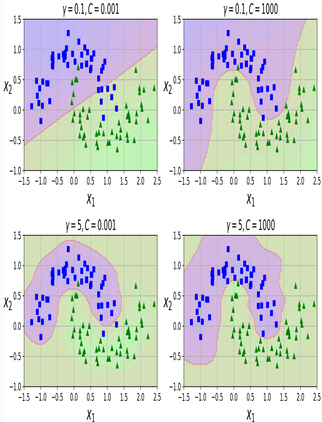
Figure 5-9. SVM classifiers using an RBF kernel
