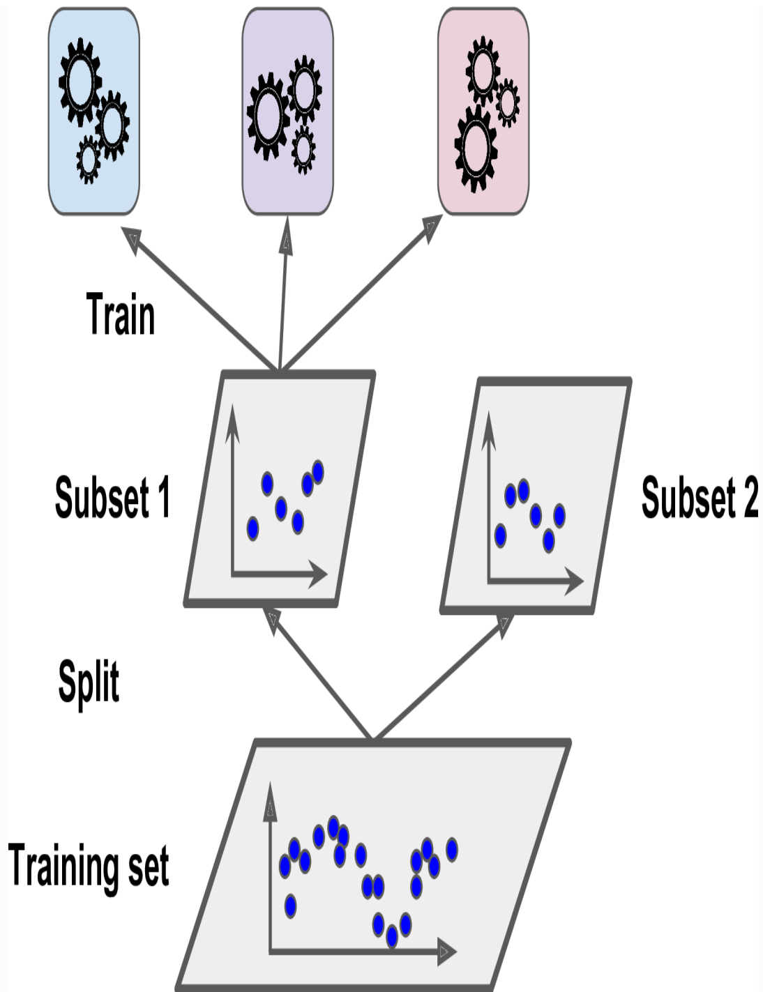
Figure 7-13. Training the first layer
