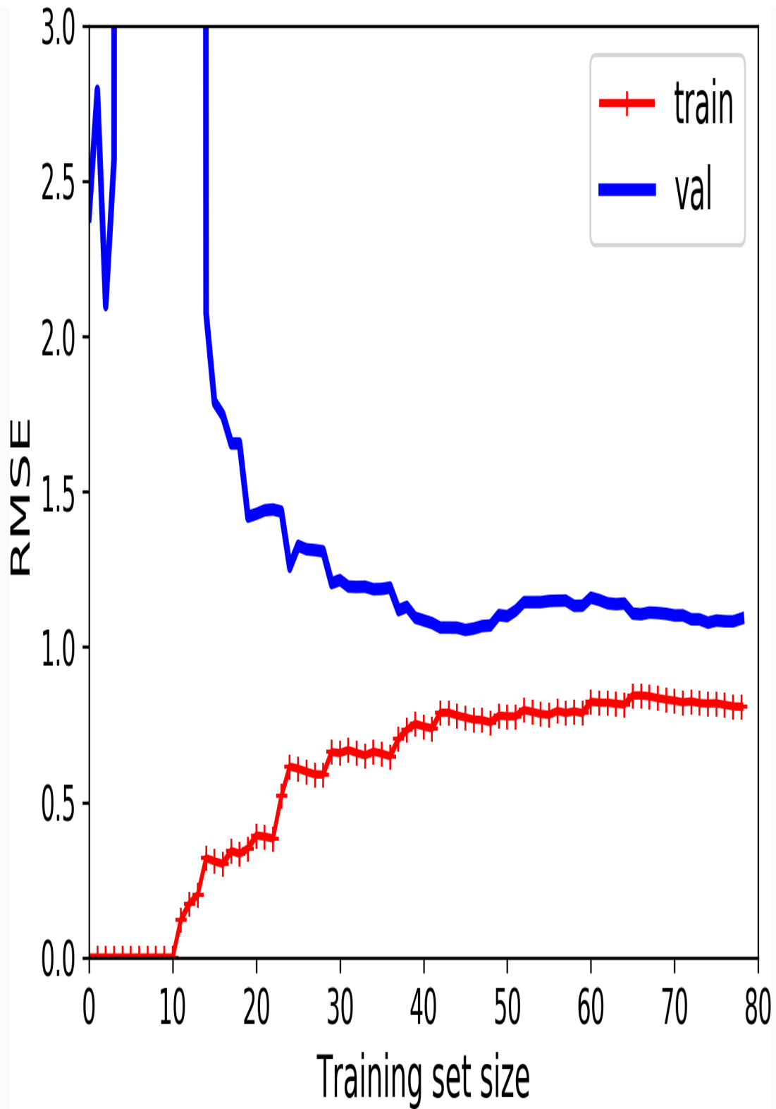
Figure 4-16. Learning curves for the polynomial model
