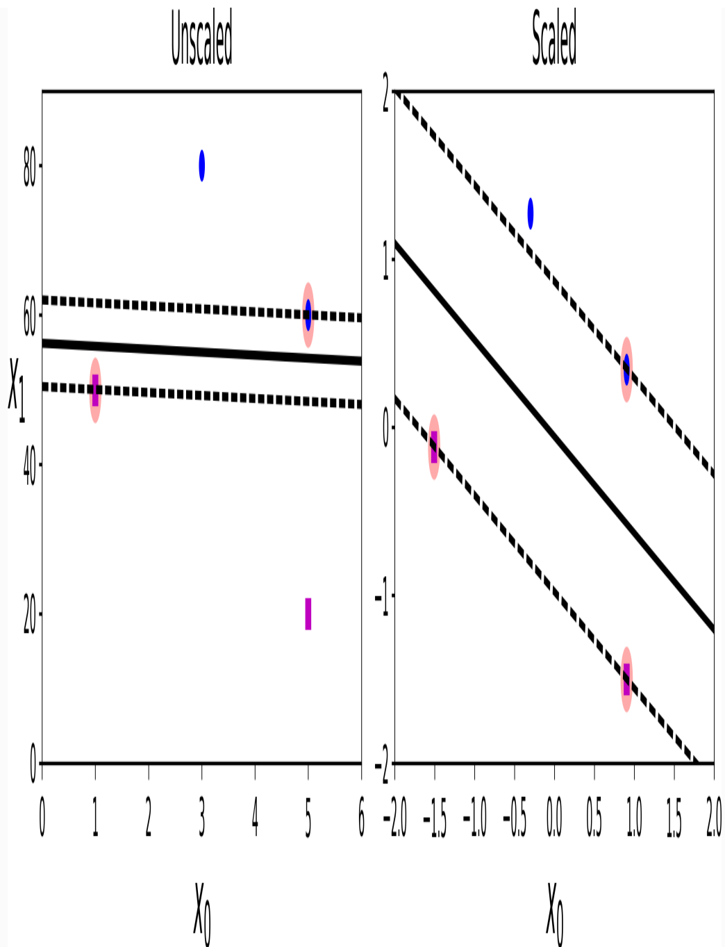
Figure 5-2. Sensitivity to feature scales
