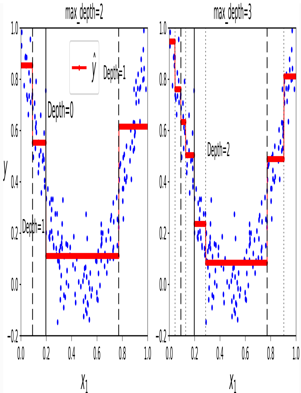
Figure 6-5. Predictions of two Decision Tree regression models
