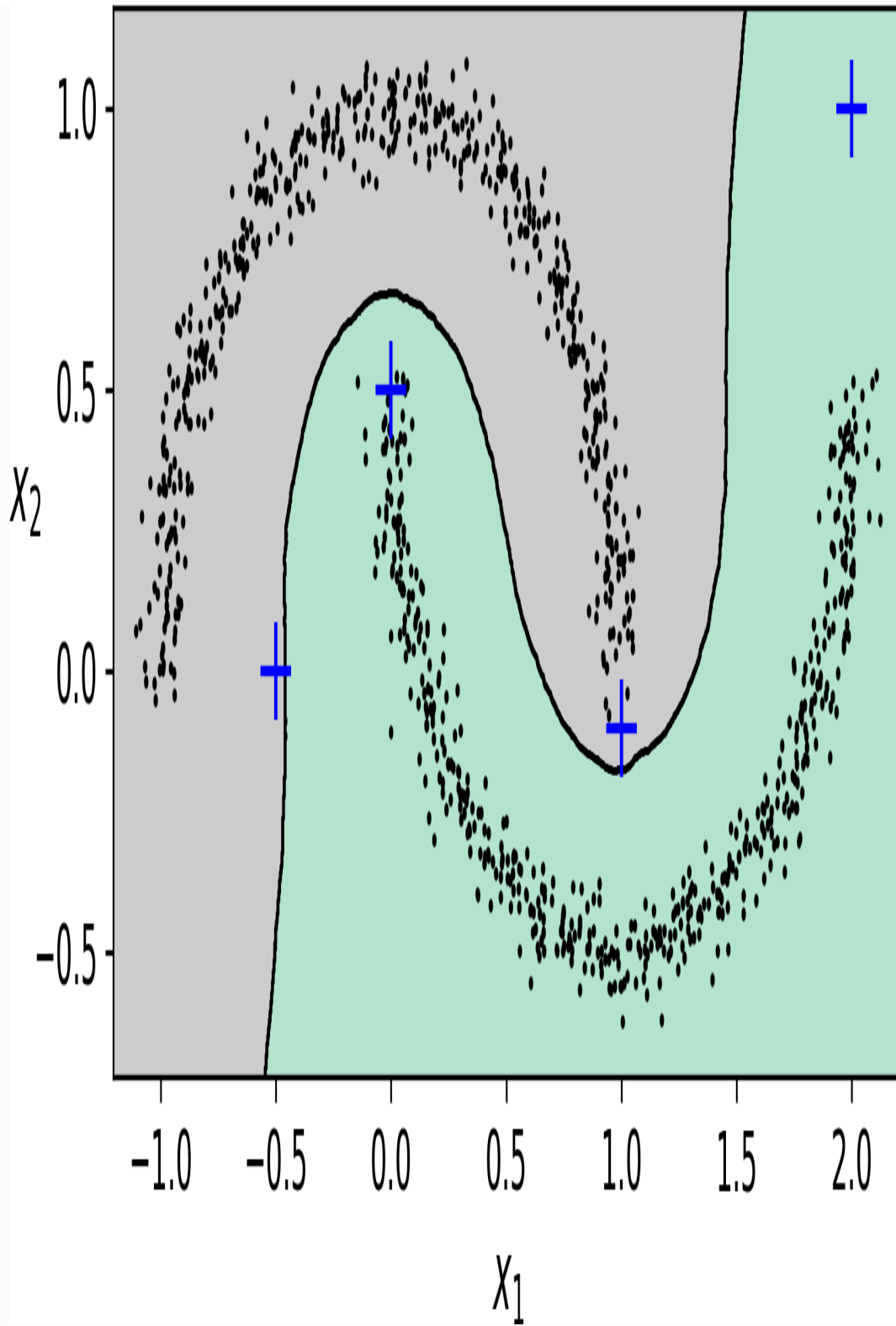
Figure 9-15. cluster_classification_diagram
