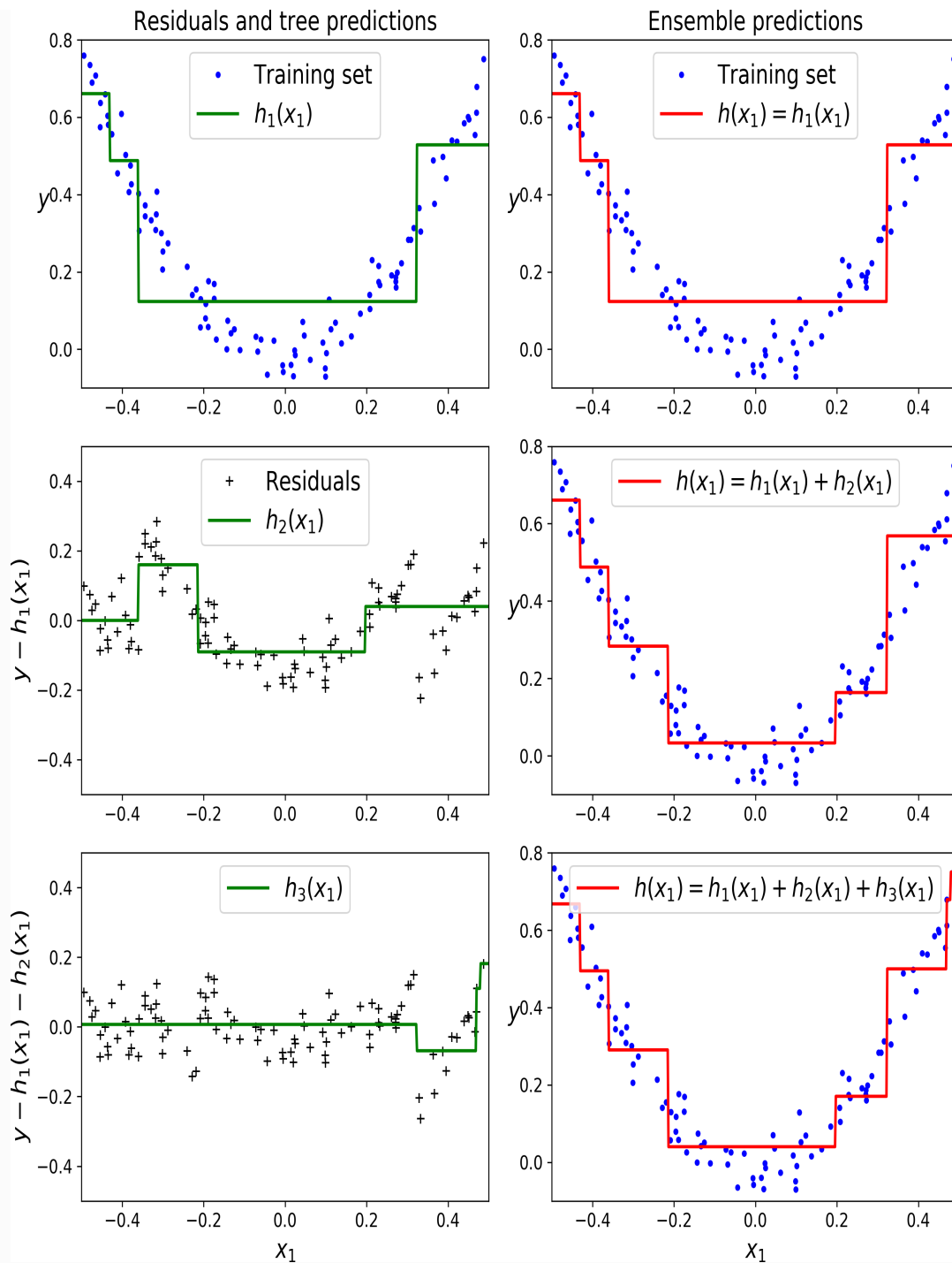
Figure 7-9. Gradient Boosting
