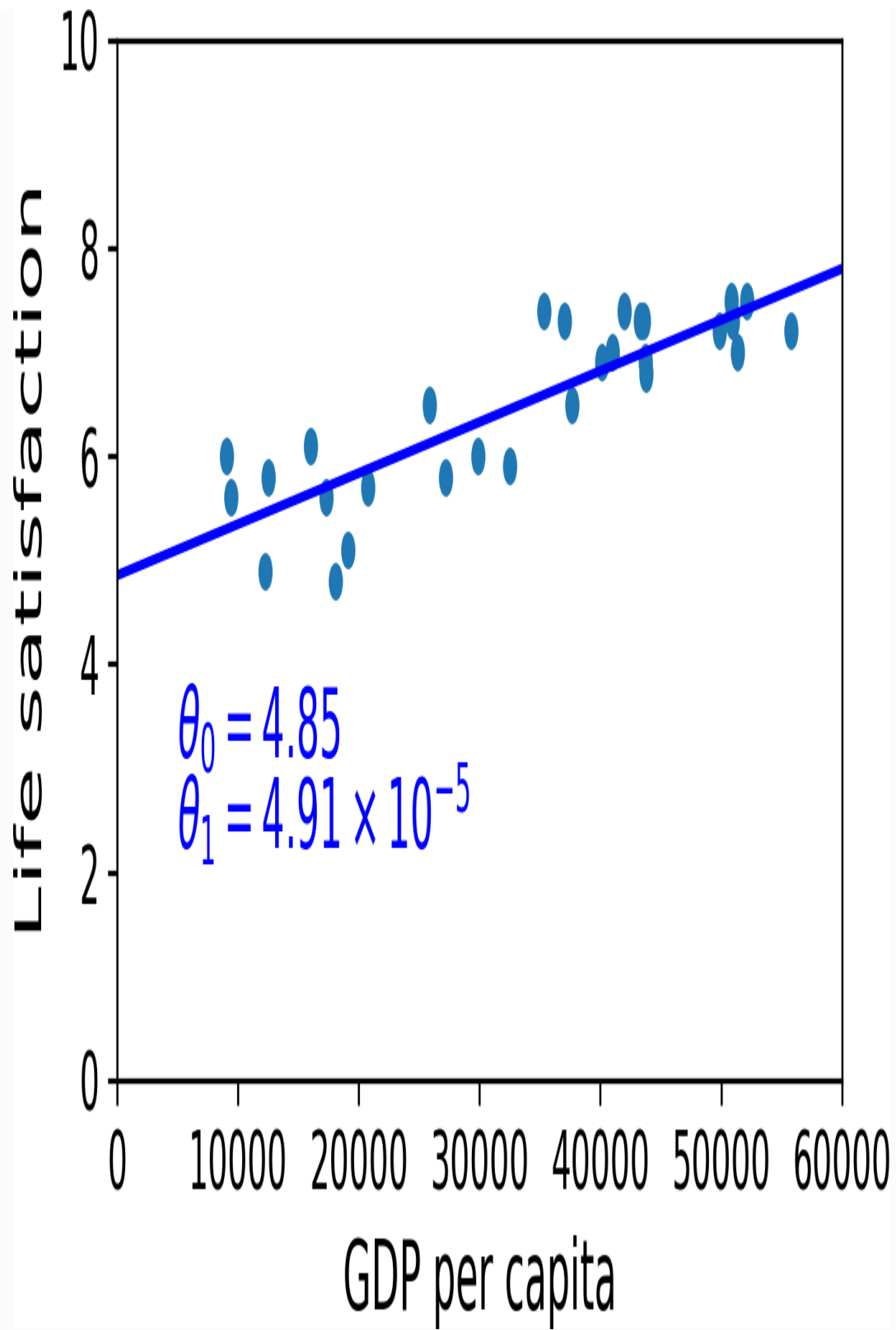
Figure 1-19. The linear model that fits the training data best
