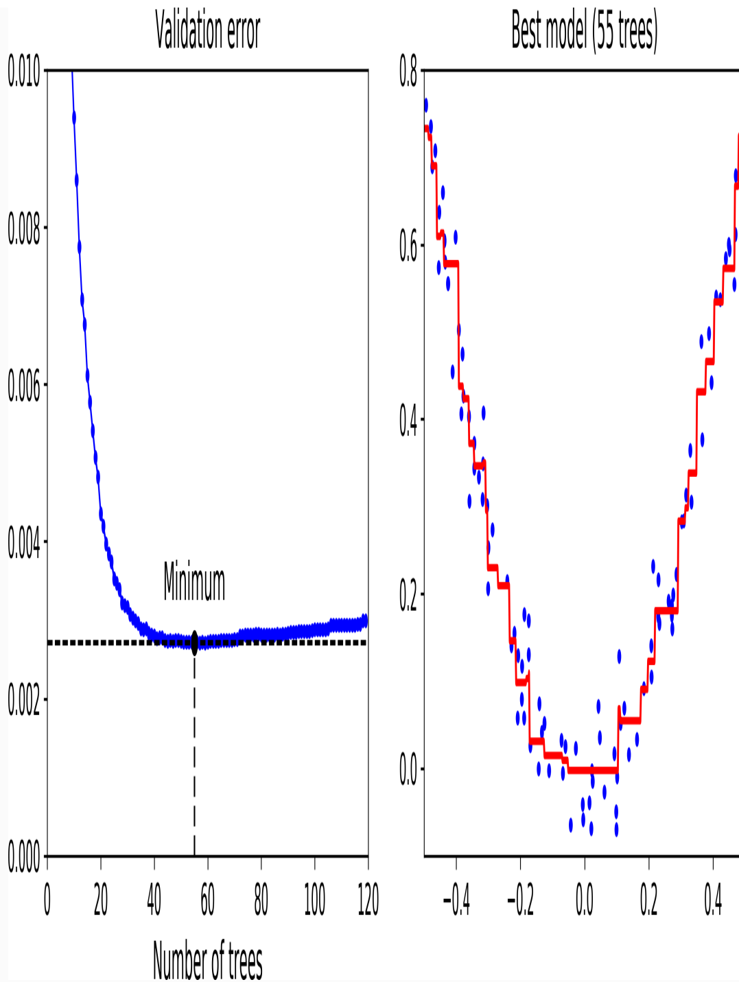
Figure 7-11. Tuning the number of trees using early stopping
