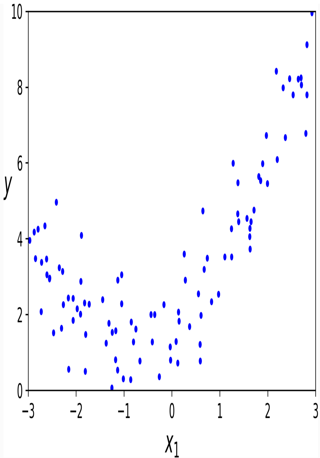
Figure 4-12. Generated nonlinear and noisy dataset
