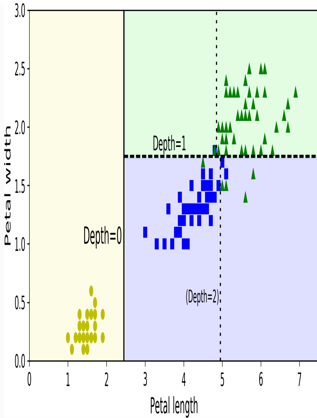
Figure 6-2. Decision Tree decision boundaries
