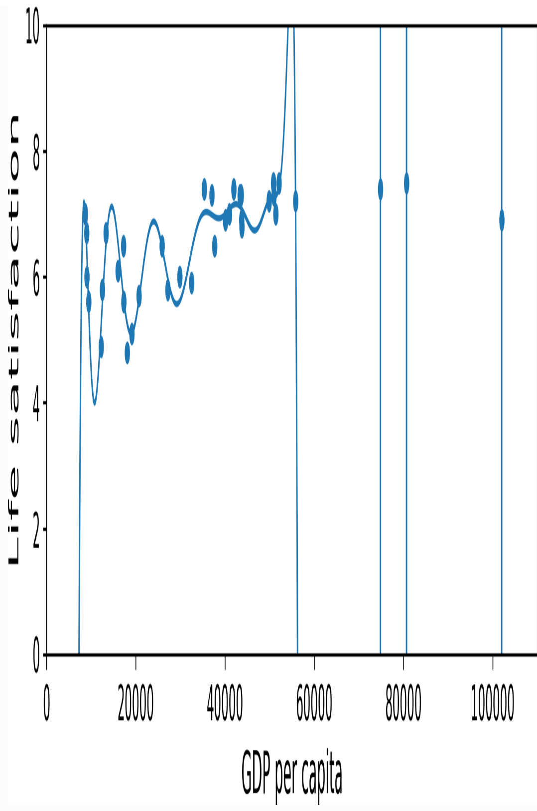
Figure 1-22. Overfitting the training data
