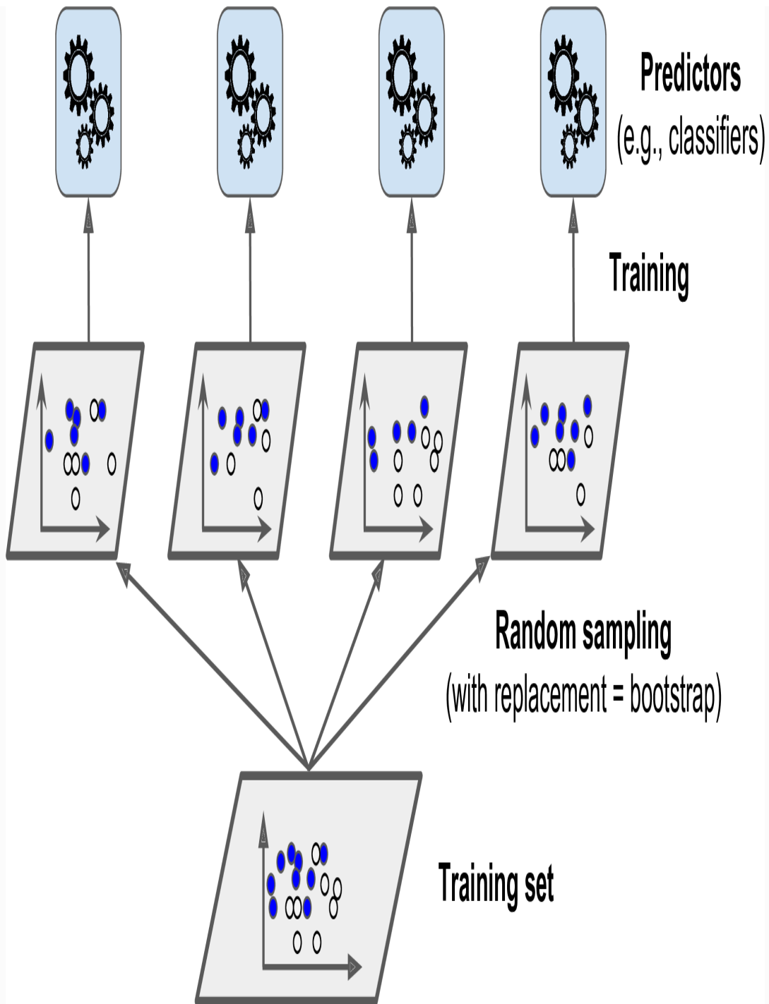
Figure 7-4. Pasting/bagging training set sampling and training
