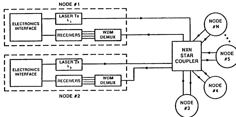
Figure 8.5: Schematic of the Lambda network with N nodes. Each node consists of one transmitter and N receivers. (After Ref. [28]; ©1990 IEEE; reprinted with permission.)
