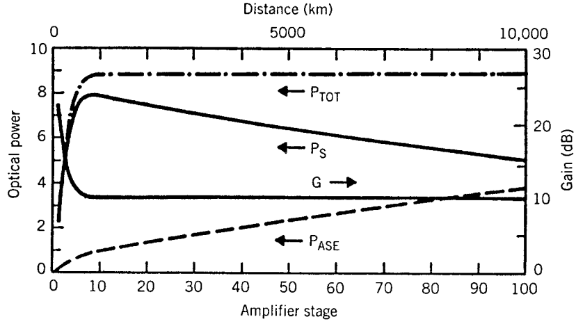
Figure 6.21: Variation of the signal power P_s and the ASE power P_{\text{ASE}} along a cascaded chain of optical amplifiers. The total power P_{\text{TOT}} becomes nearly constant after a few amplifiers. (After Ref. [119]; ©1991 IEEE; reprinted with permission.)
