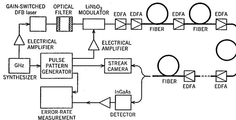
Figure 9.13: Setup used for soliton transmission in a 1990 experiment. Two EDFAs after the LiNbO 3 modulator boost pulse peak power to the level of fundamental solitons. (After Ref. [70]; ©1990 IEEE; reprinted with permission.)
