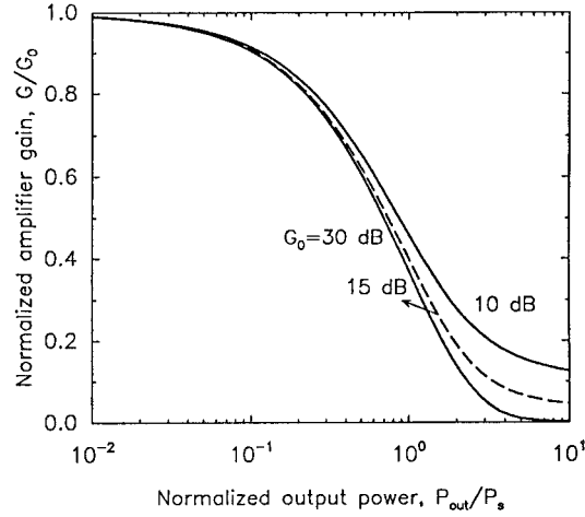
Figure 6.2: Saturated amplifier gain G as a function of the output power (normalized to the saturation power) for several values of the unsaturated amplifier gain G_0 .
