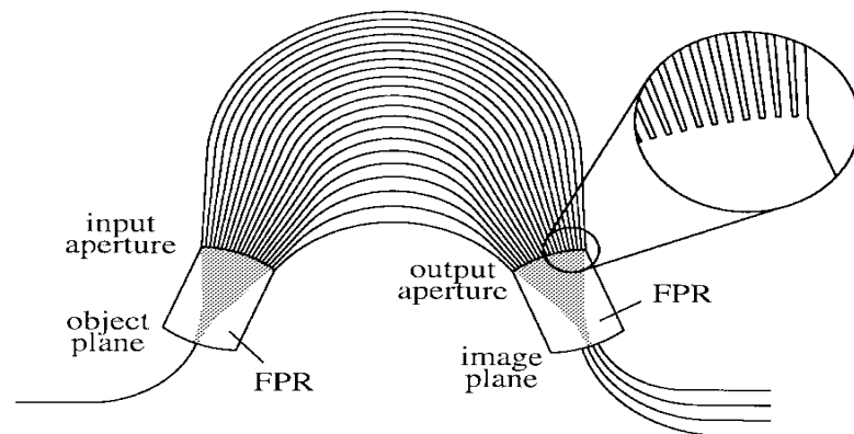
Figure 8.11: Schematic of a waveguide-grating demultiplexer consisting of an array of waveguides between two free-propagation regions (FPR). (After Ref. [74]; ©1996 IEEE; reprinted with permission.)
