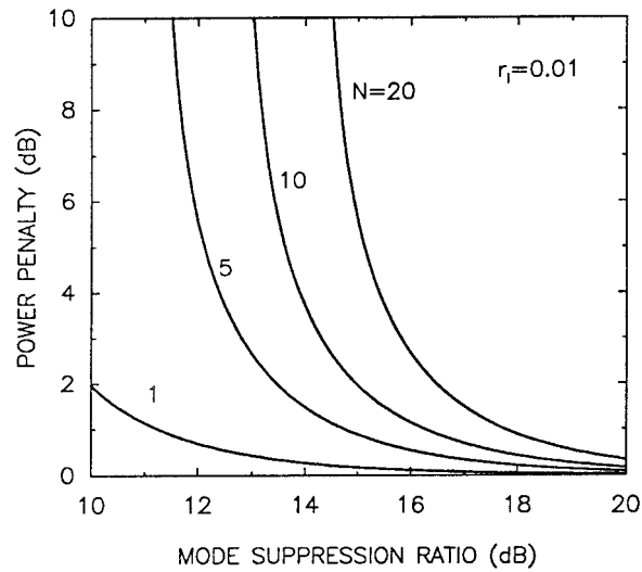
Figure 5.14: Feedback-induced power penalty as a function of MSR for several values of N and r_f = 0.01 . Reflection feedback into the laser is assumed to generate N side modes of the same amplitude.
