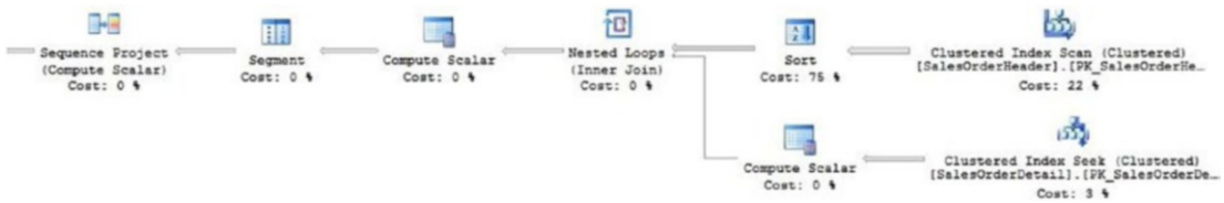
Figure 8-9. Execution plan for a search that uses parameterized paging
