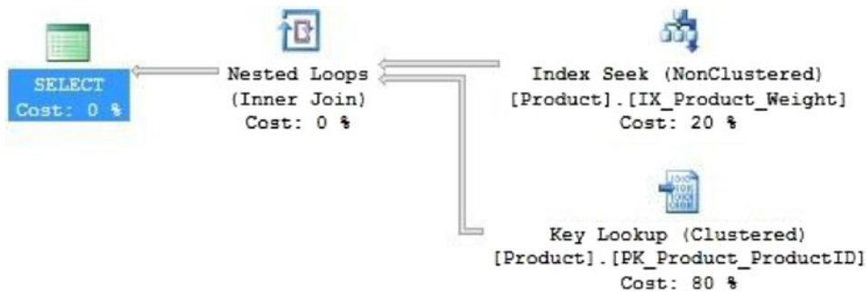
Figure 6-21. Performance of the search query against a larger result set
