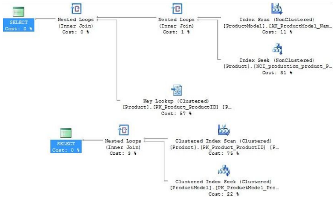
Figure 8-20. Performance of a query with a small result set variables are declared and the stored proc parameters reassigned locally
