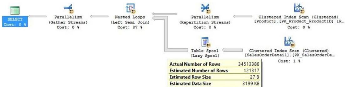
Figure 8-17. Performance of an (intentionally) poorly written query
