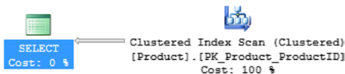
Figure 6-24. Performance of the previous search query with updated statistics
