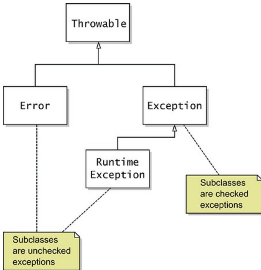
Figure 5-1 The exception hierarchy
