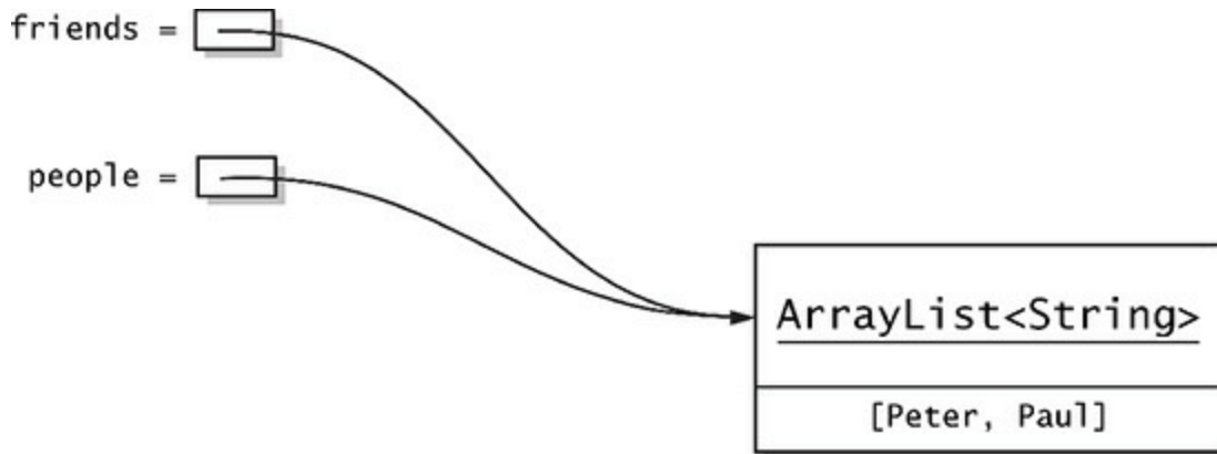
Figure 2-2 Two references to the same object
