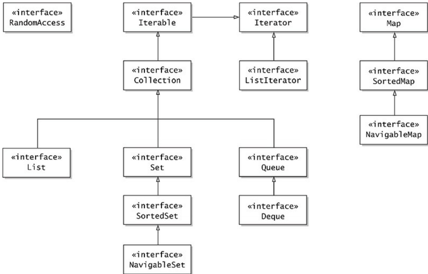
Figure 7-1 Interfaces in the Java collections framework
