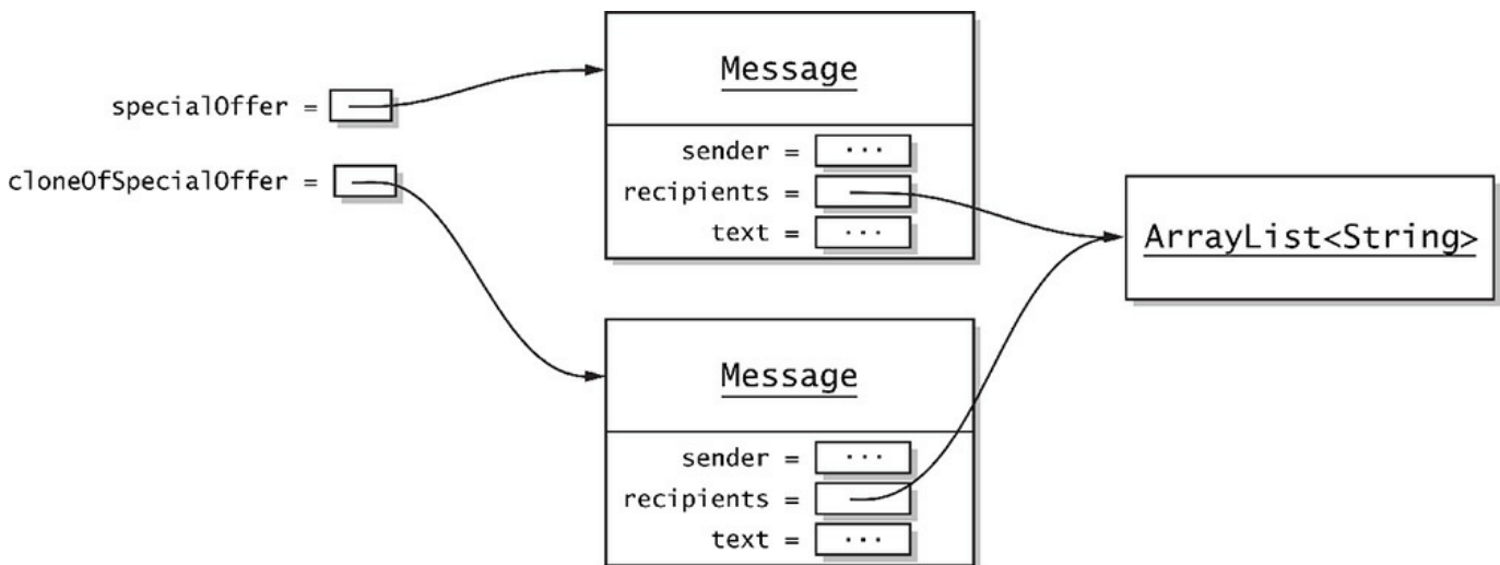
Figure 4-1 A shallow copy of an object
