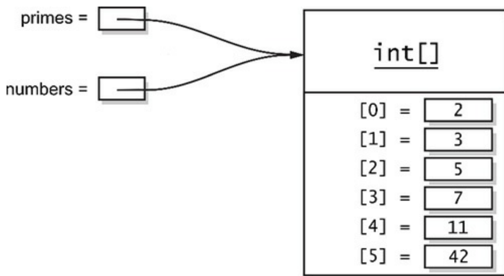
Figure 1-6 Two variables referencing the same array
