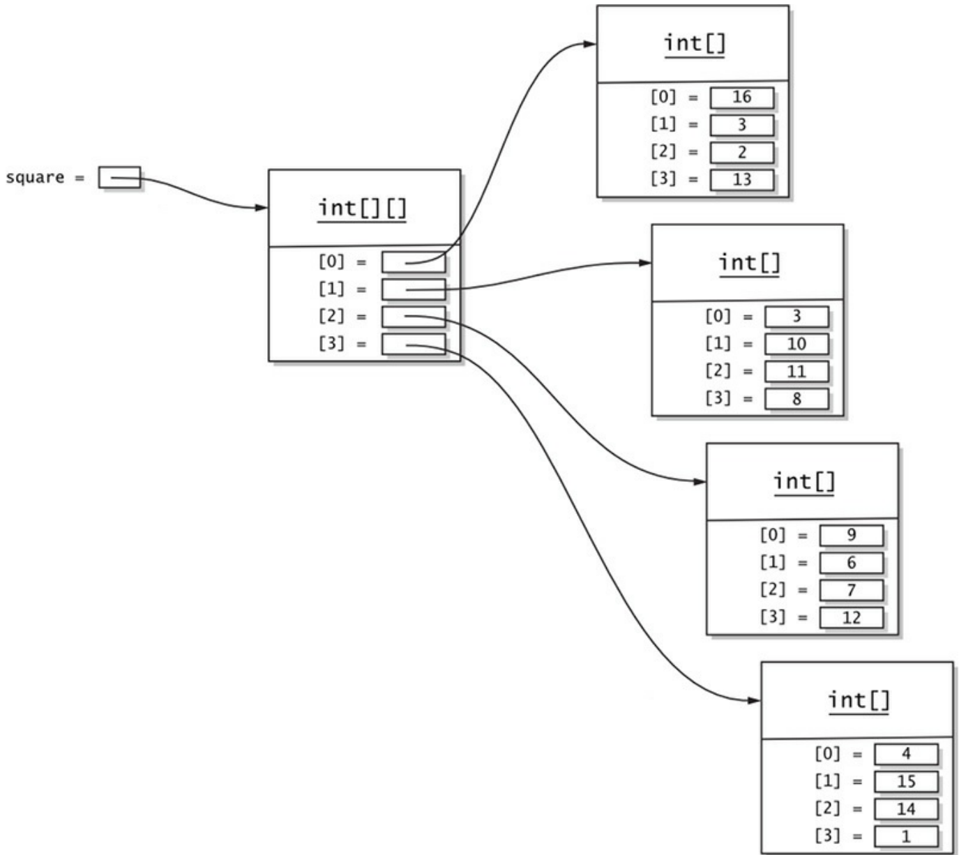
Figure 1-7 A two-dimensional array
