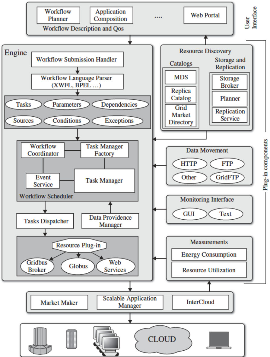
FIGURE 12.2. Architecture of Workflow Management System.
