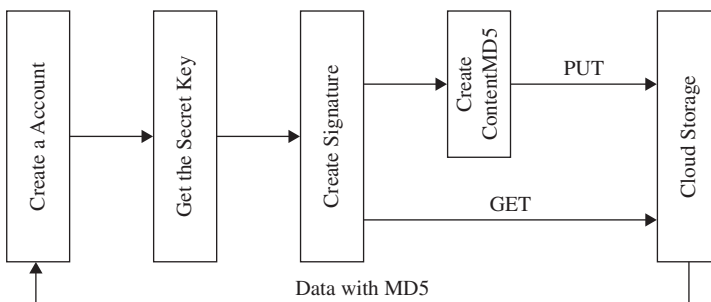
FIGURE 8.3. Security data access procedure.
