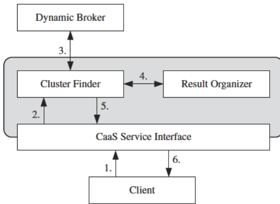
FIGURE 7.9. Cluster discovery.
