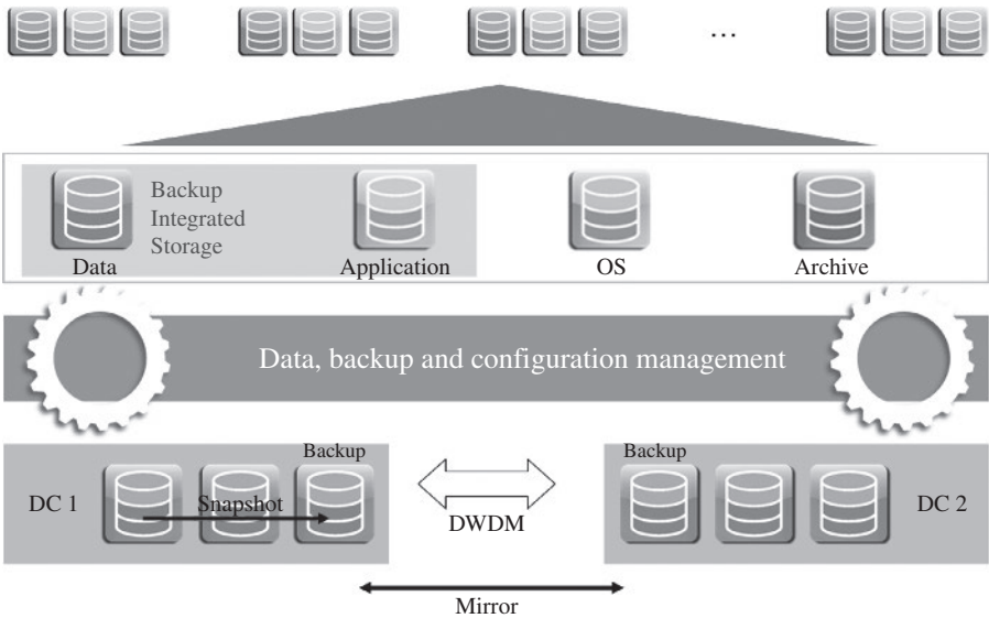
FIGURE 11.4. Storage resources: backup integrated, read only, and archive storage.
