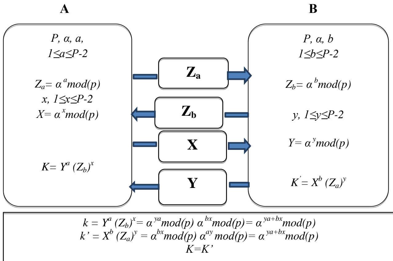
3.18- rasm. MTI protokoli
