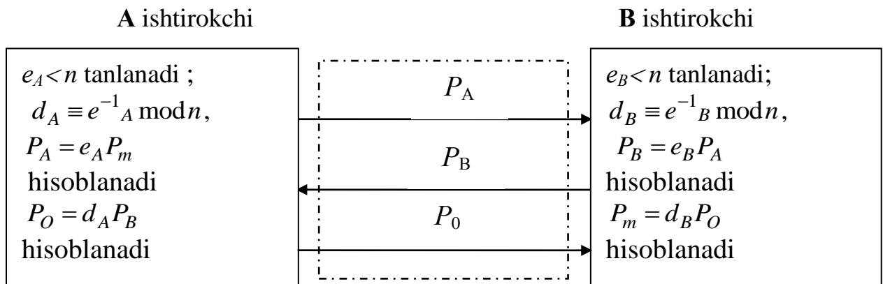
3.23- rasm. Messi – Omur sxemasi bo‘yicha kalit taqsimlash protokoli
