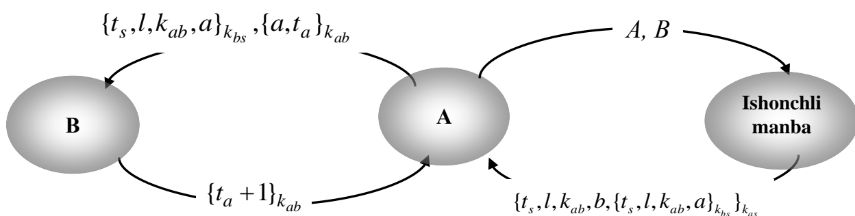
2.2- rasm. Kerberos protokoli
