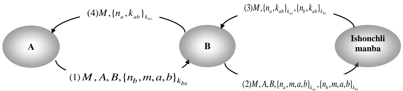
3.12- rasm. Otvey-Riis protokoli
