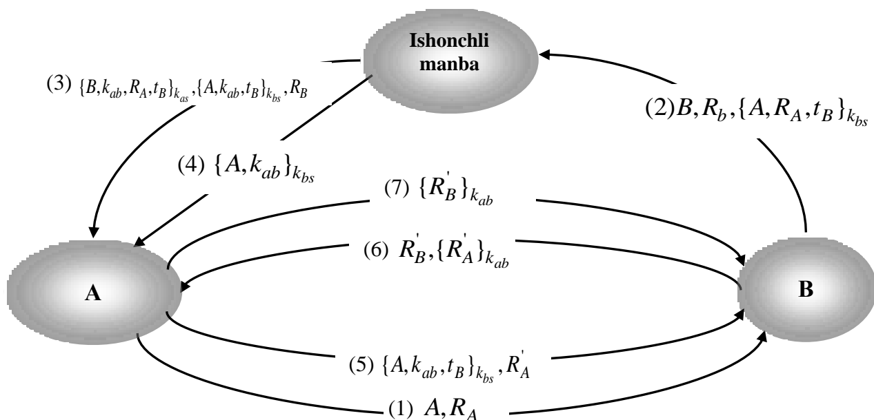
3.14- rasm. Nyuman-Stabblbayn protokoli
