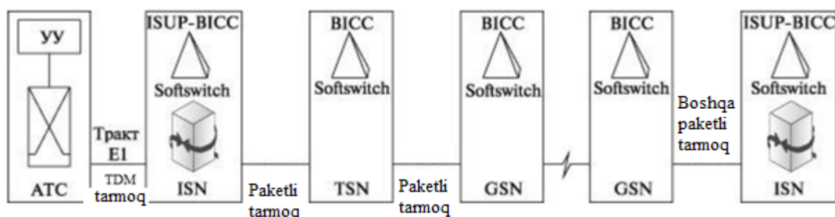
8.4-rasm. BICC protokolinig ishlash tamoili
