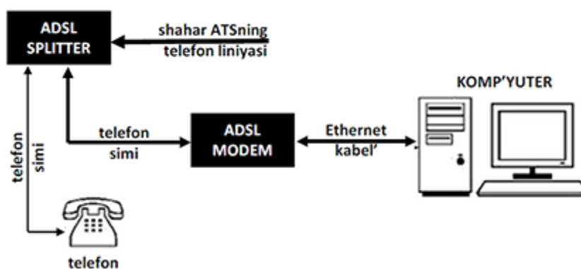
9.6-rasm. Abonent inshootida ADSL tarmog'ining oddiy ulanish sxemasi
