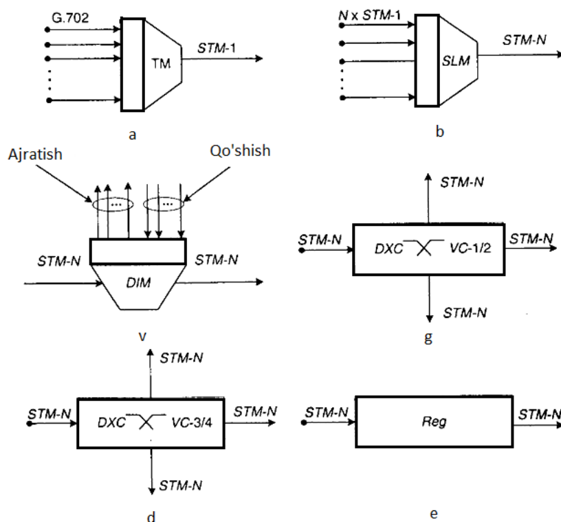
5.1 – rasm. TM (a,b), ADM (v), DXC(g,d) va regeneratlarning shartli (e) belgilanishlari
