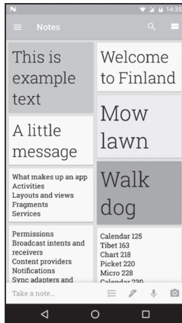
StaggeredGridLayoutManager
