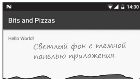
Theme.AppCompat.Light.DarkActionBar
