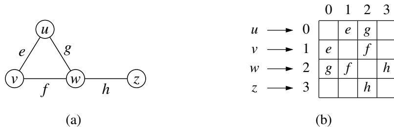
Figure 14.7: (a) An undirected graph G ; (b) a schematic representation of the auxiliary adjacency matrix structure for G , in which n vertices are mapped to indices 0 to n - 1 . Although not diagrammed as such, we presume that there is a unique Edge instance for each edge, and that it maintains references to its endpoint vertices. We also assume that there is a secondary edge list (not pictured), to allow the edges() method to run in O(m) time, for a graph with m edges.
