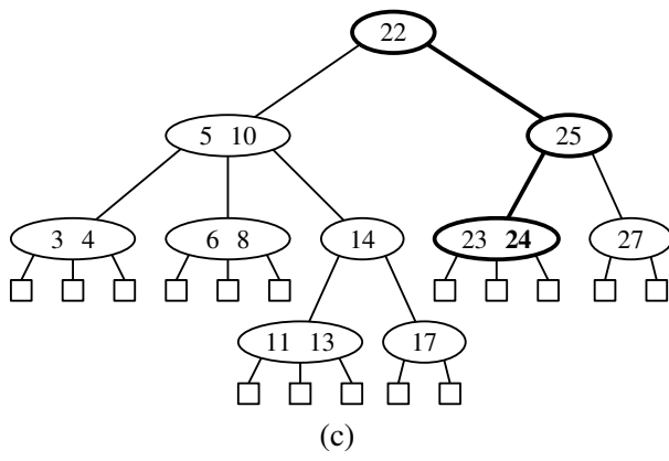
Figure 11.23: (a) A multiway search tree T ; (b) search path in T for key 12 (unsuccessful search); (c) search path in T for key 24 (successful search).
