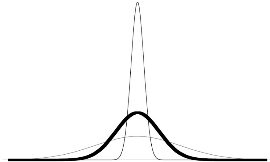
FIGURE 7: How the Law of Large Numbers Works
