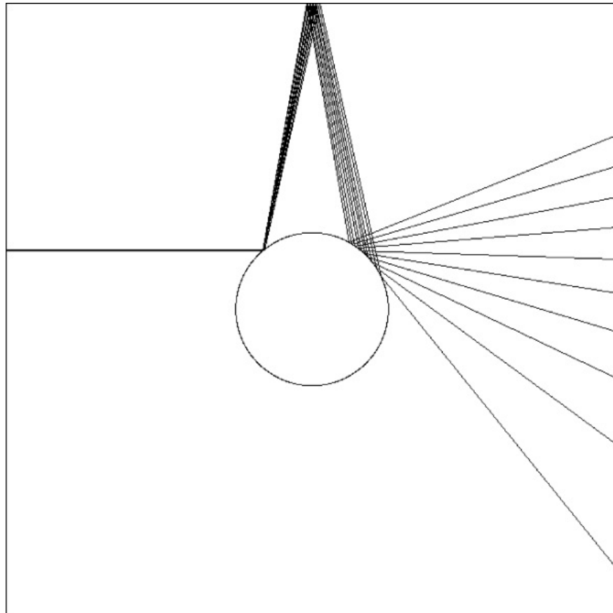
FIGURE 2: PRECISION AND FORECASTING
