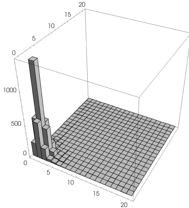
FIGURE 13: THE PURE FRACTAL STATISTICAL MOUNTAIN
