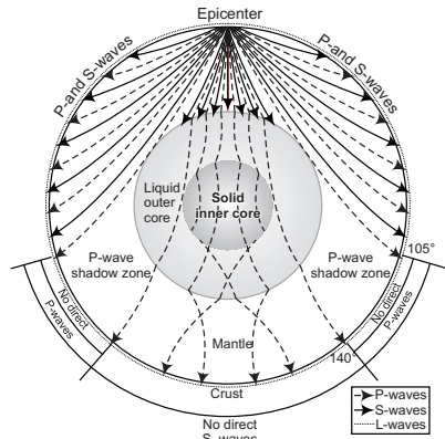
Earthquake Waves
