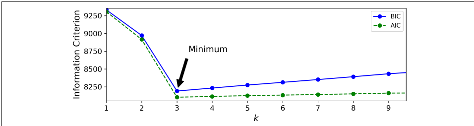
Figure 9-21. AIC and BIC for different numbers of clusters k
