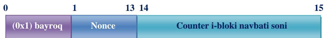
4.34- rasm. CBR bloki
